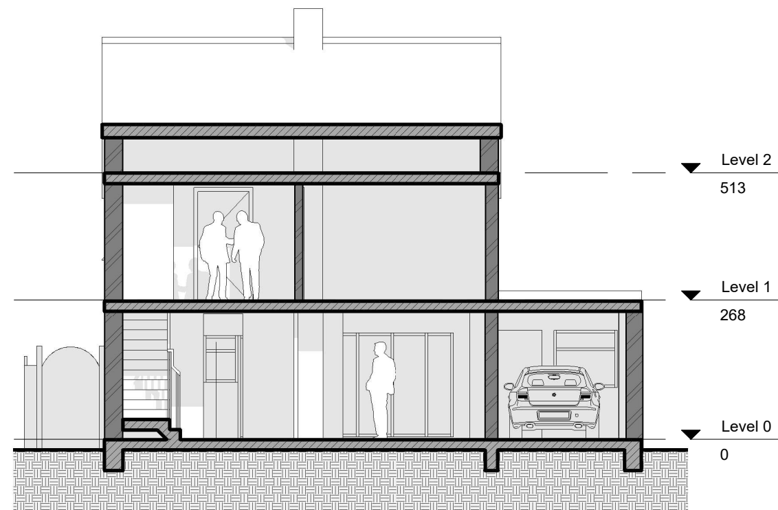
Existing Cross Section 1:100
