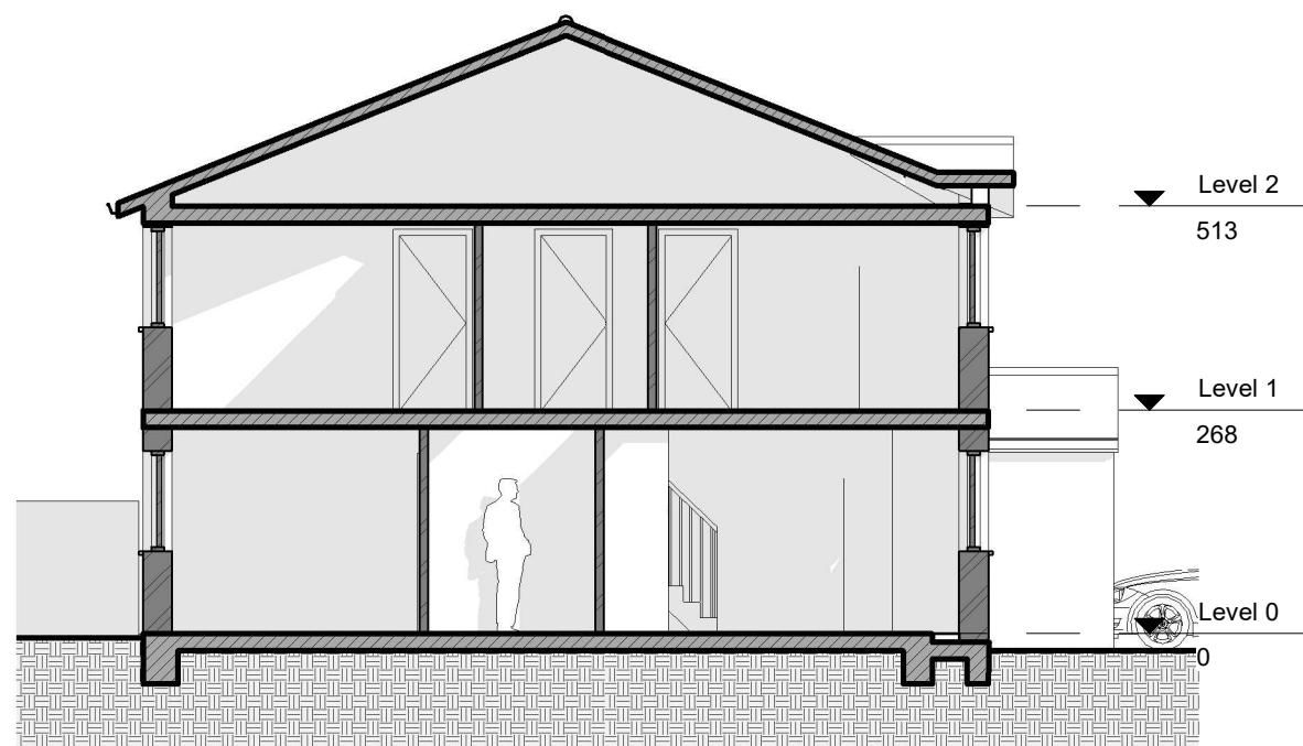
Proposed Longitudinal Section 1:100
