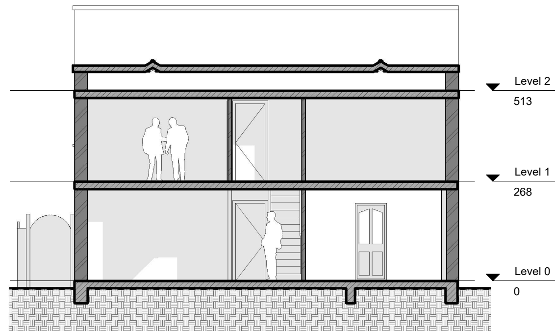
Proposed Cross Section 1:100
