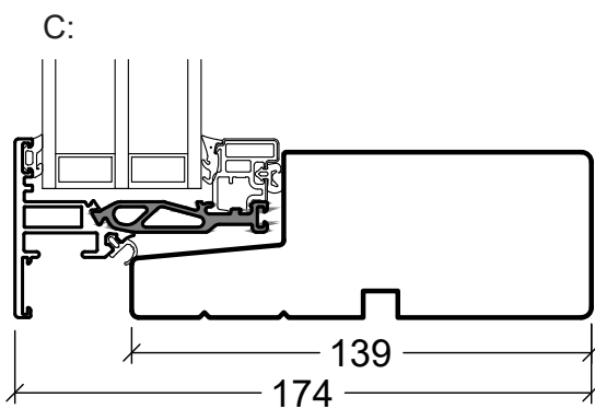
139mm frame
