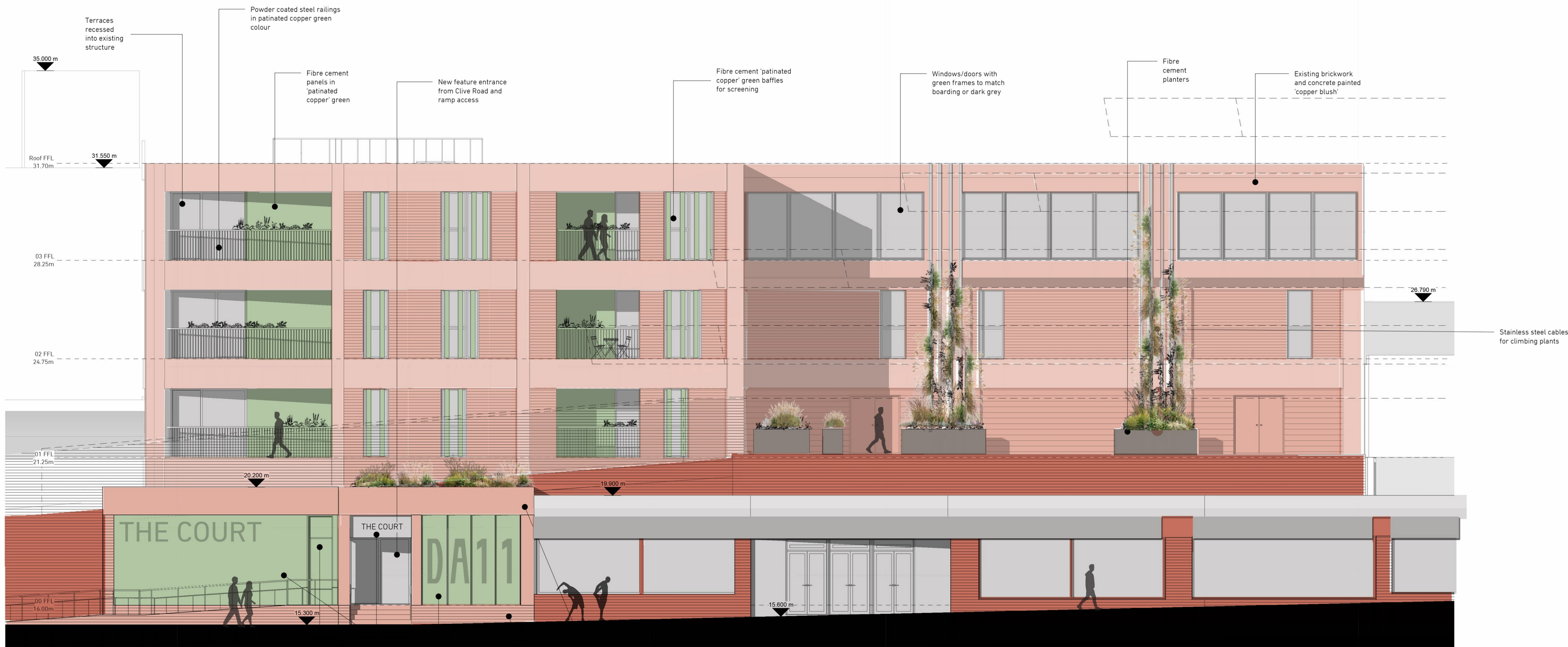
1 Elevation G Rear Block - Clive Road 1 : 100
