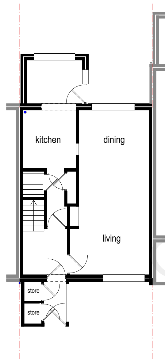
ground floor plan 48 sqm
