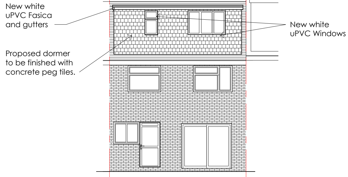
PROPOSED BACK ELEVATION
