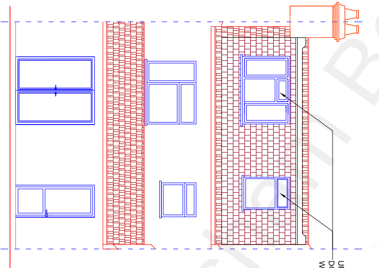
UPVC FRAMED DOUBLE GLAZED WINDOWS
