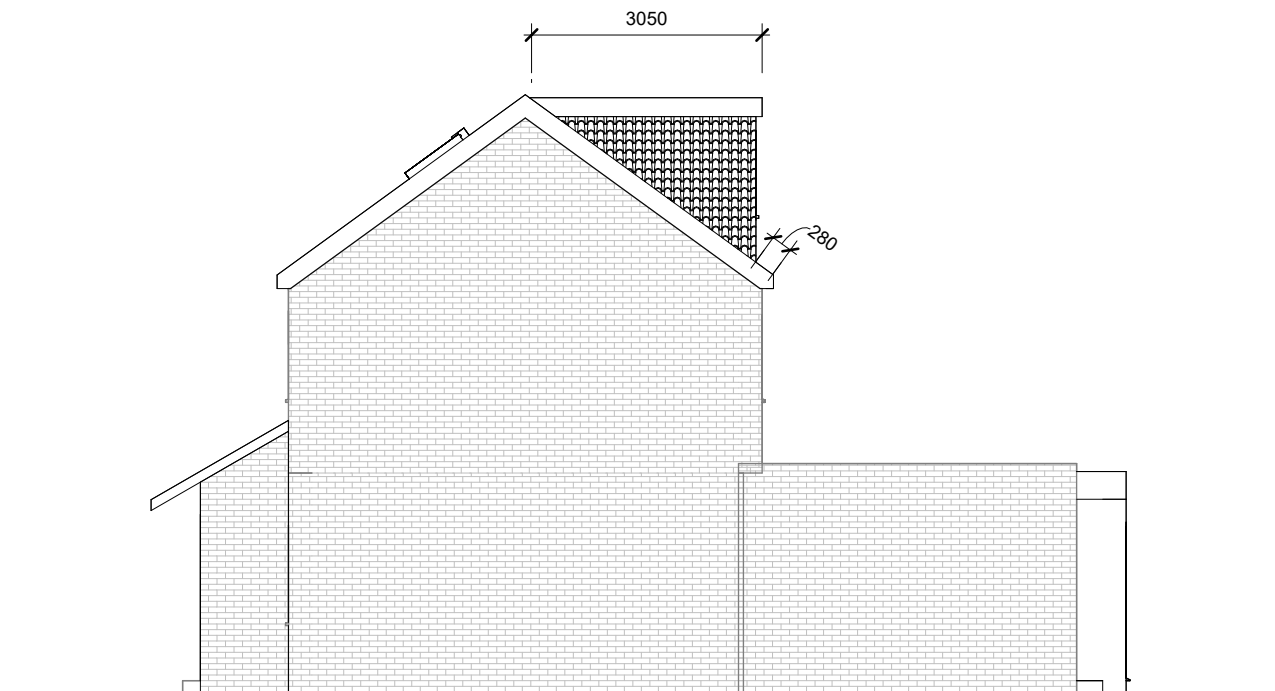
East - Proposed 1 : 100
