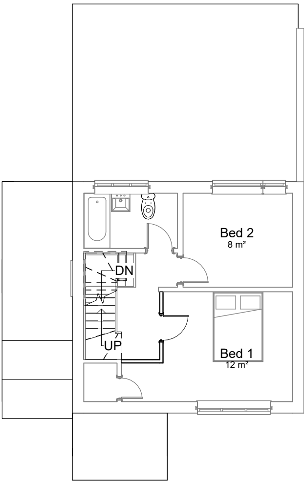
FF - Proposed 1 : 100
