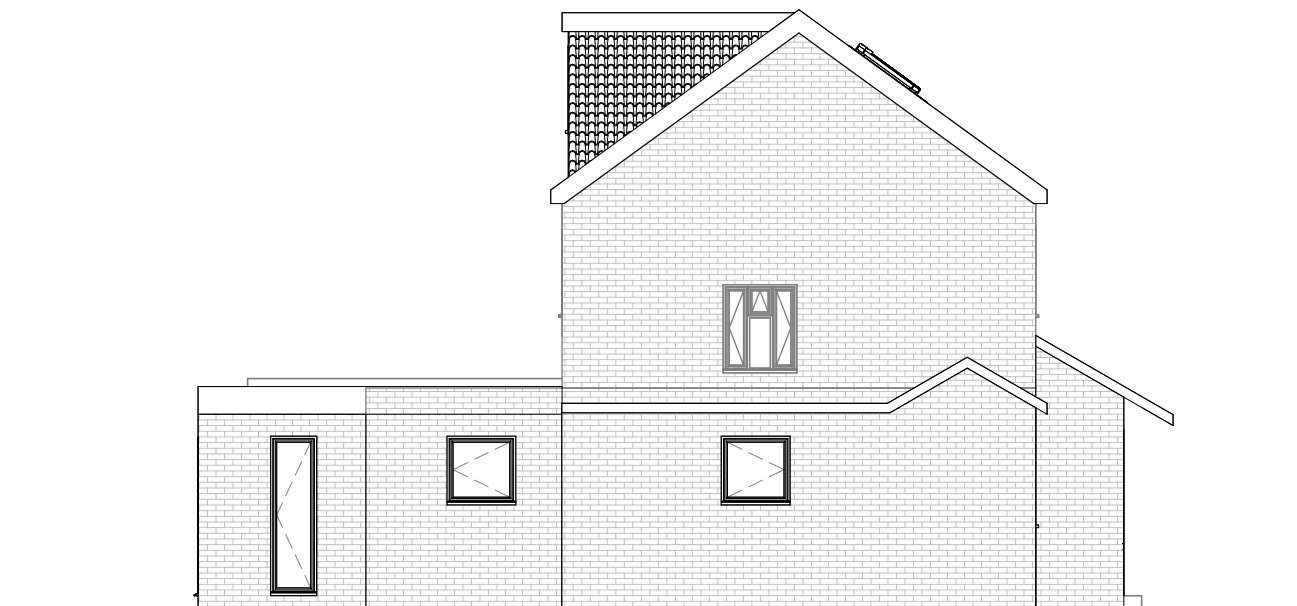
West - Proposed 1 : 100
