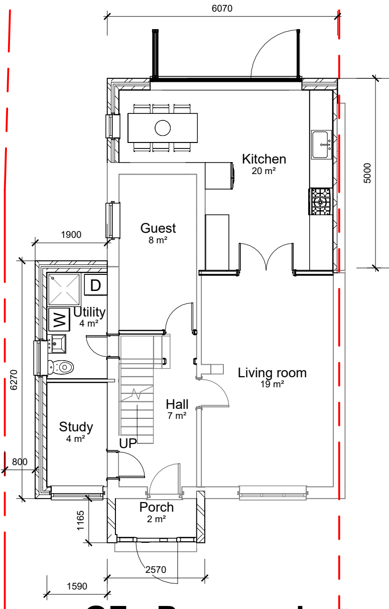
GF - Proposed 1 : 100
