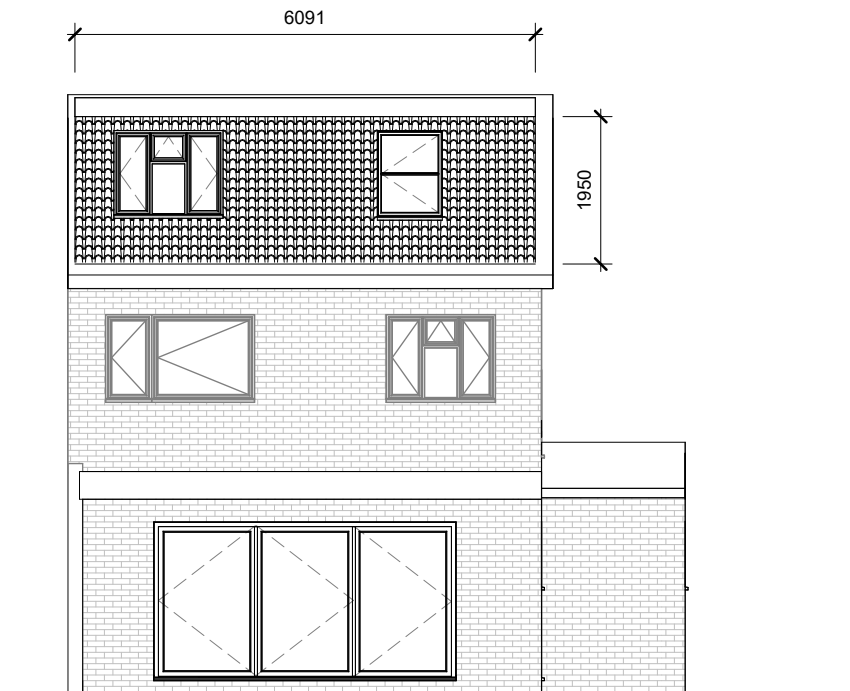
North - Proposed 1 : 100
