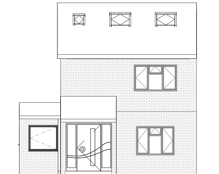
South - Proposed 1 : 100
