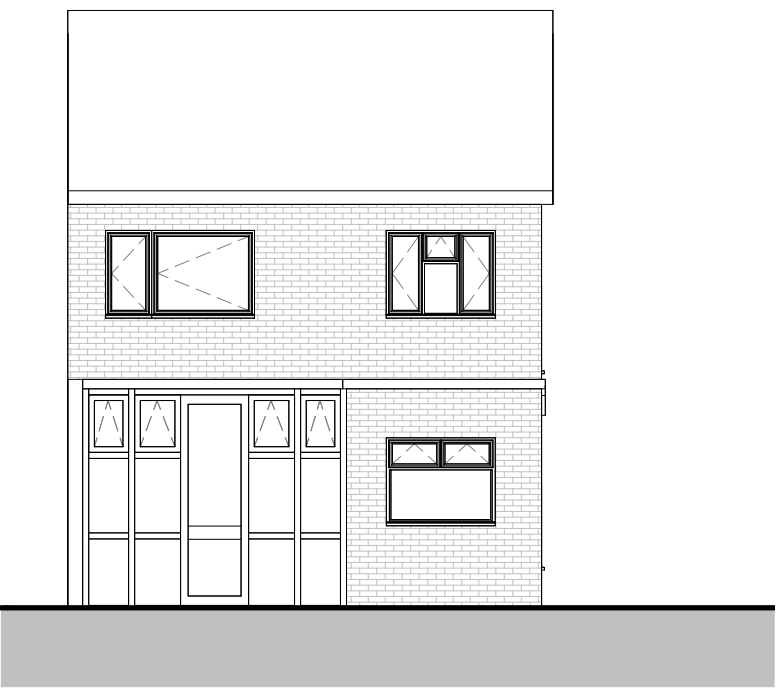
North - Existing 1 : 100
