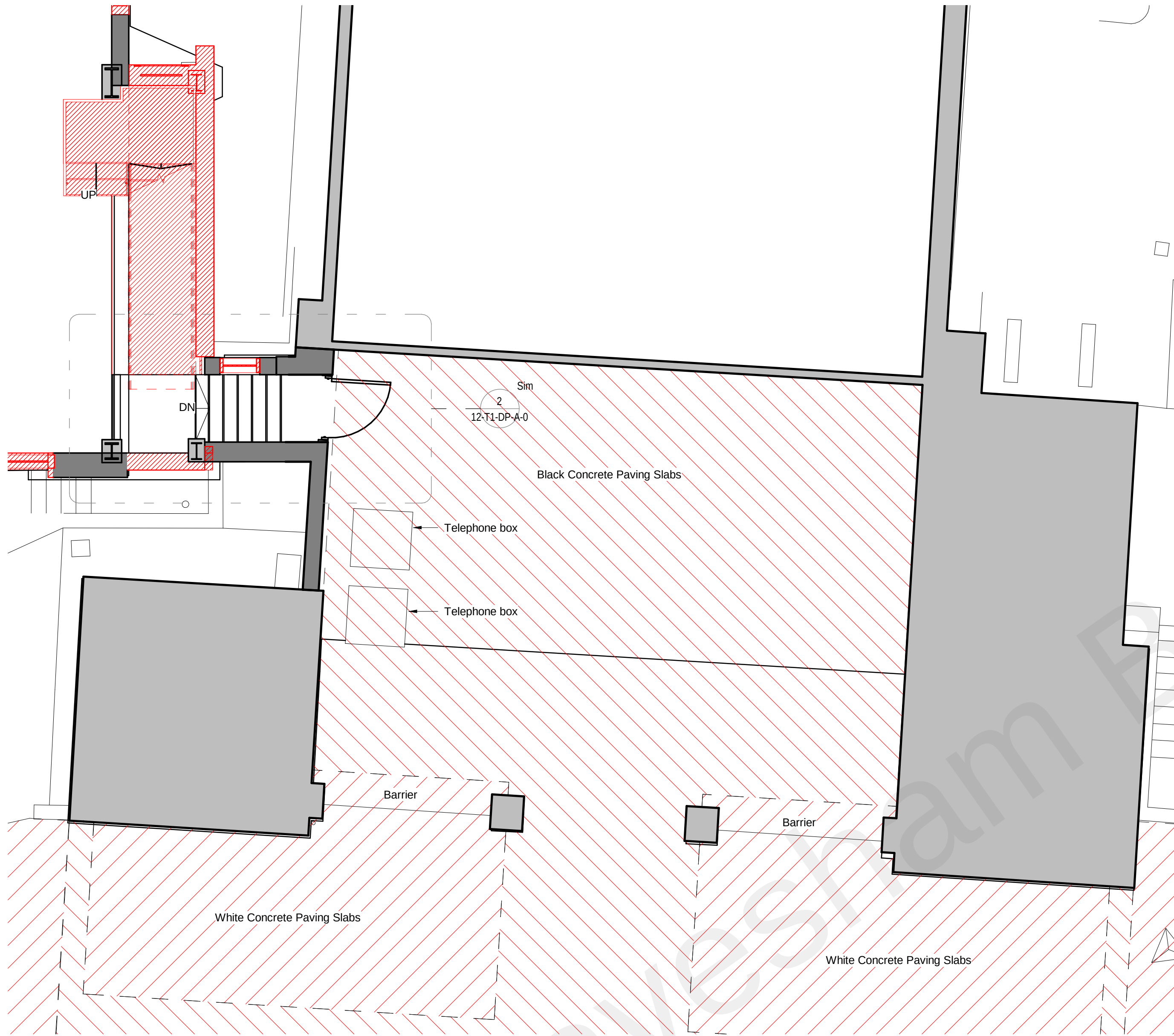
2 Existing Paving around Royal Terrace Pier 1 : 50
