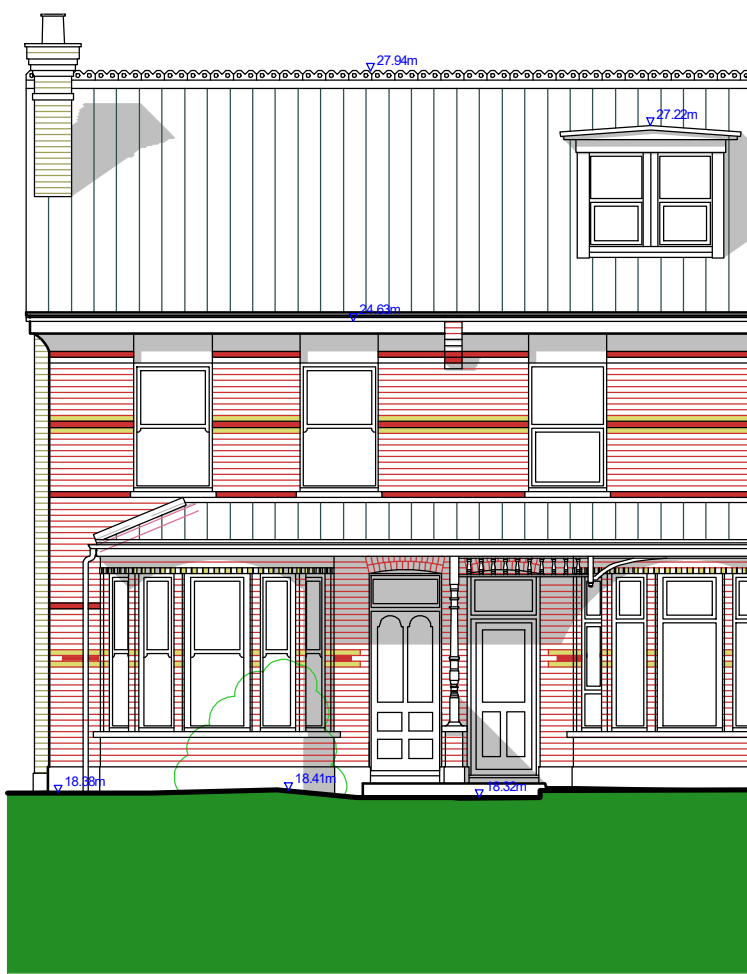
front elevation
