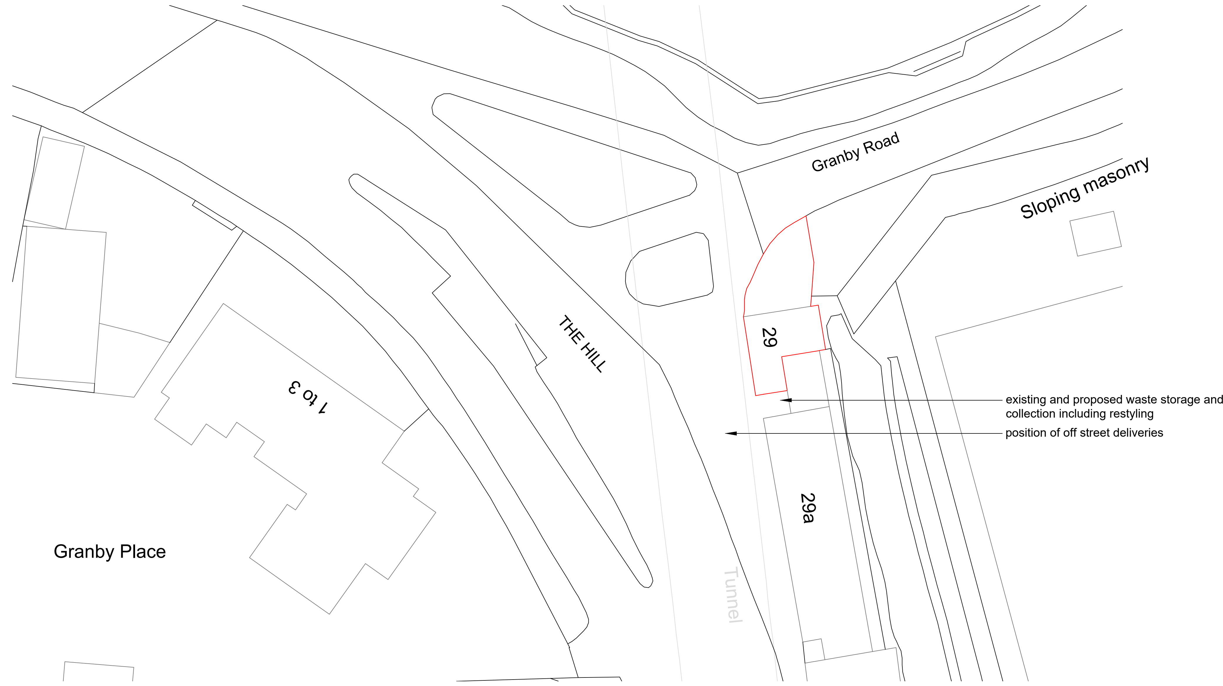
02 Existing / Proposed Block Plan Scale 1:200
