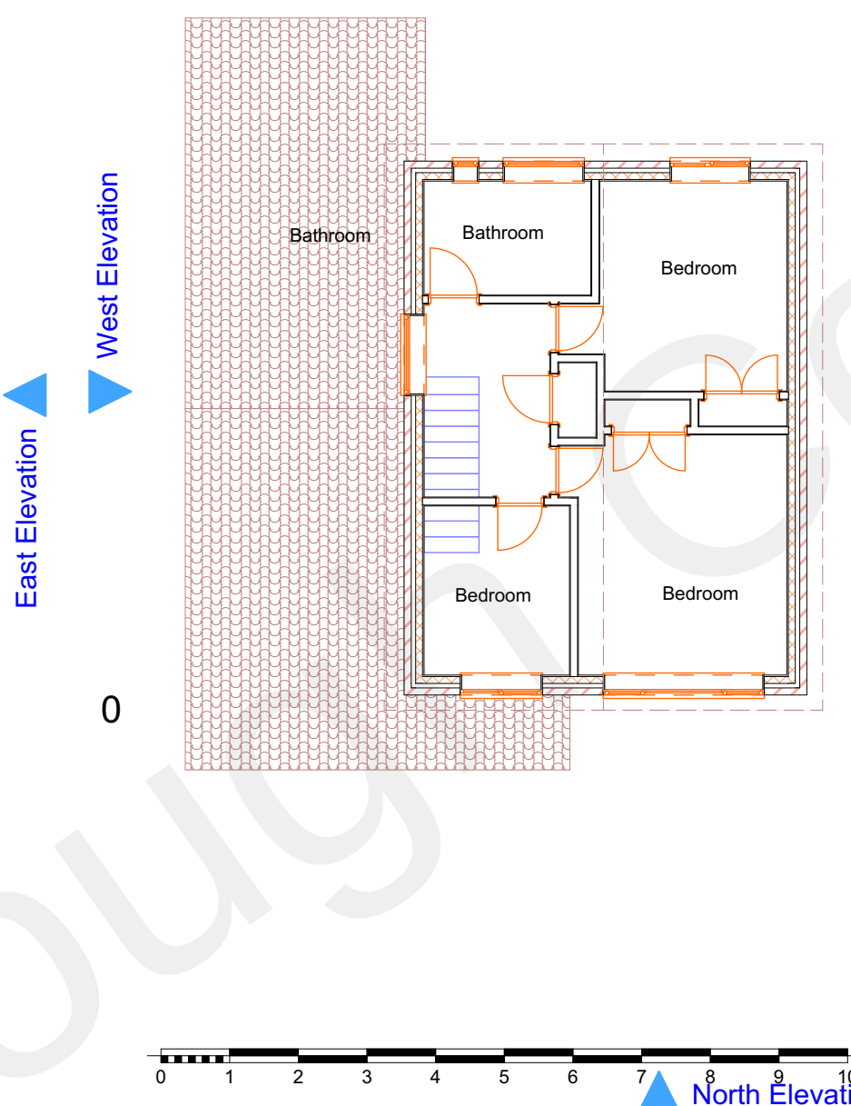
10 01 First Floor Existing 1:100
