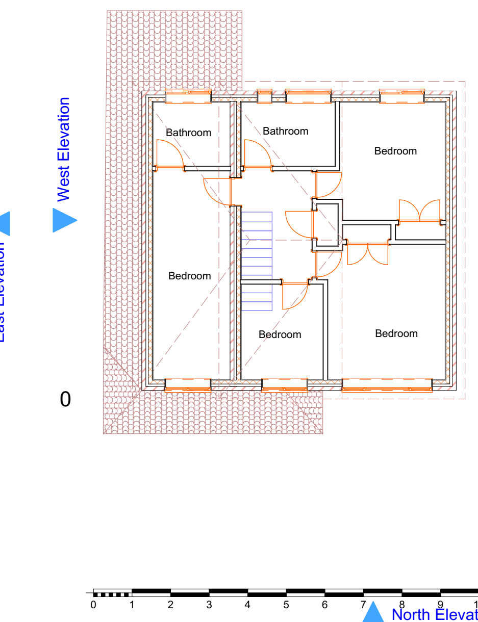
13 01 First Floor Proposed 1:100
