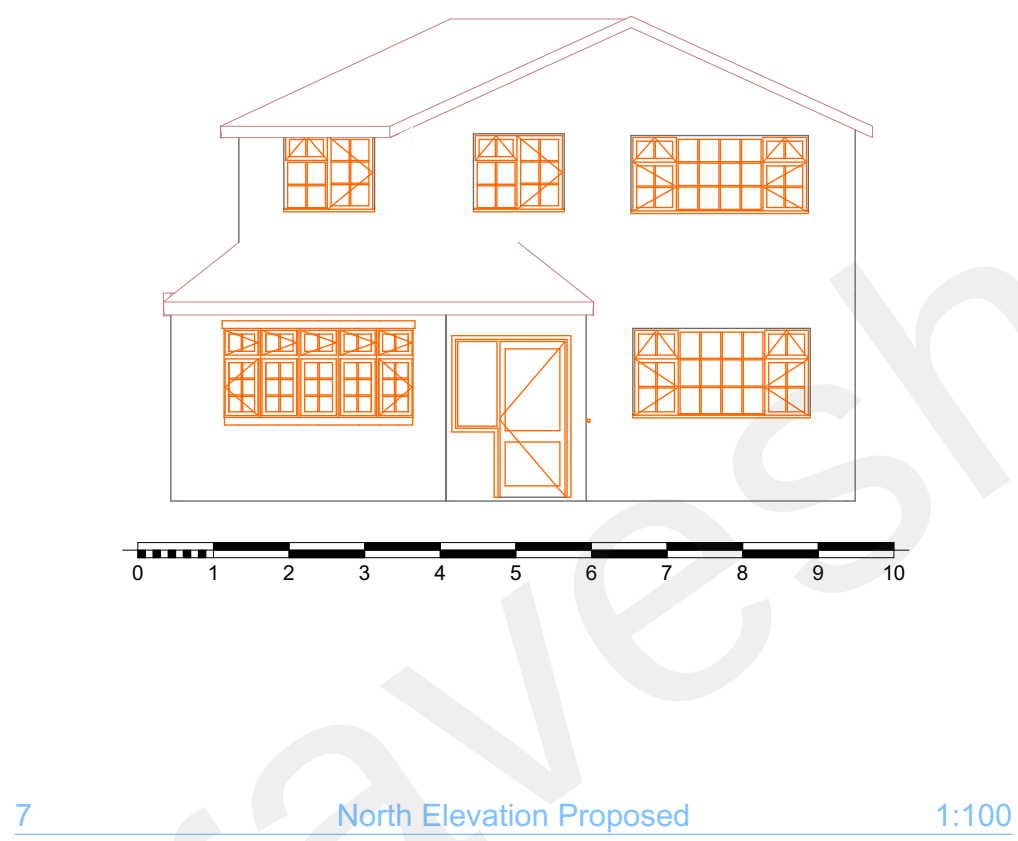
7 North Elevation Proposed 1:100
