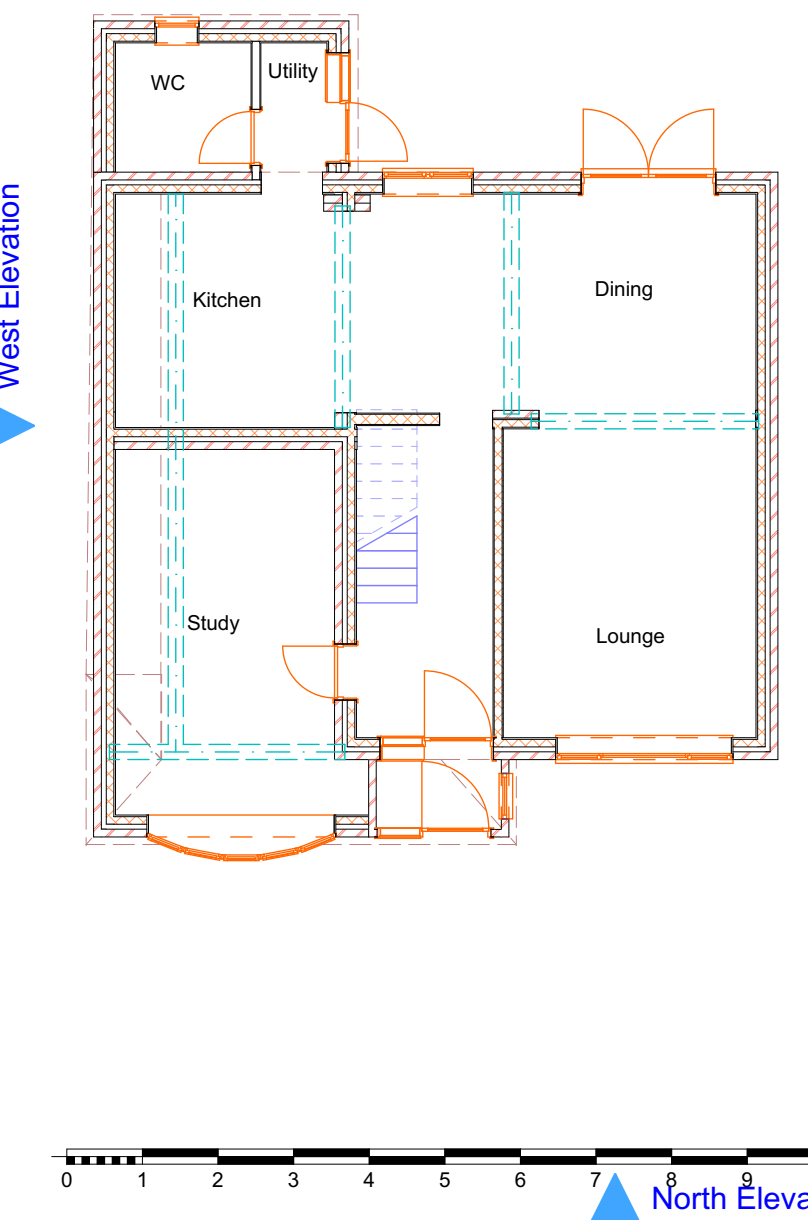
12 GF Ground Floor Proposed 1:100
