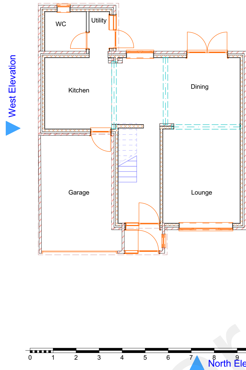
9 GF Ground Floor Existing 1:100
