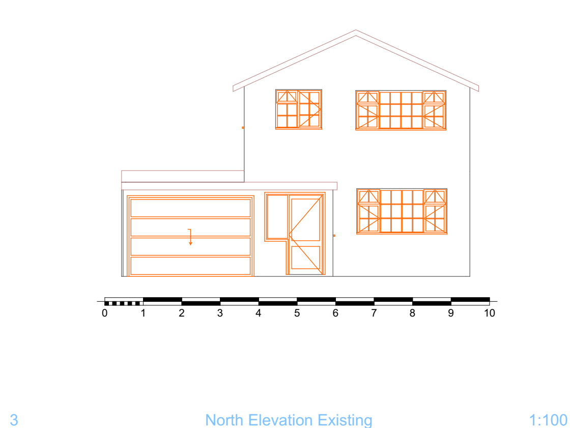
3 North Elevation Existing 1:100
