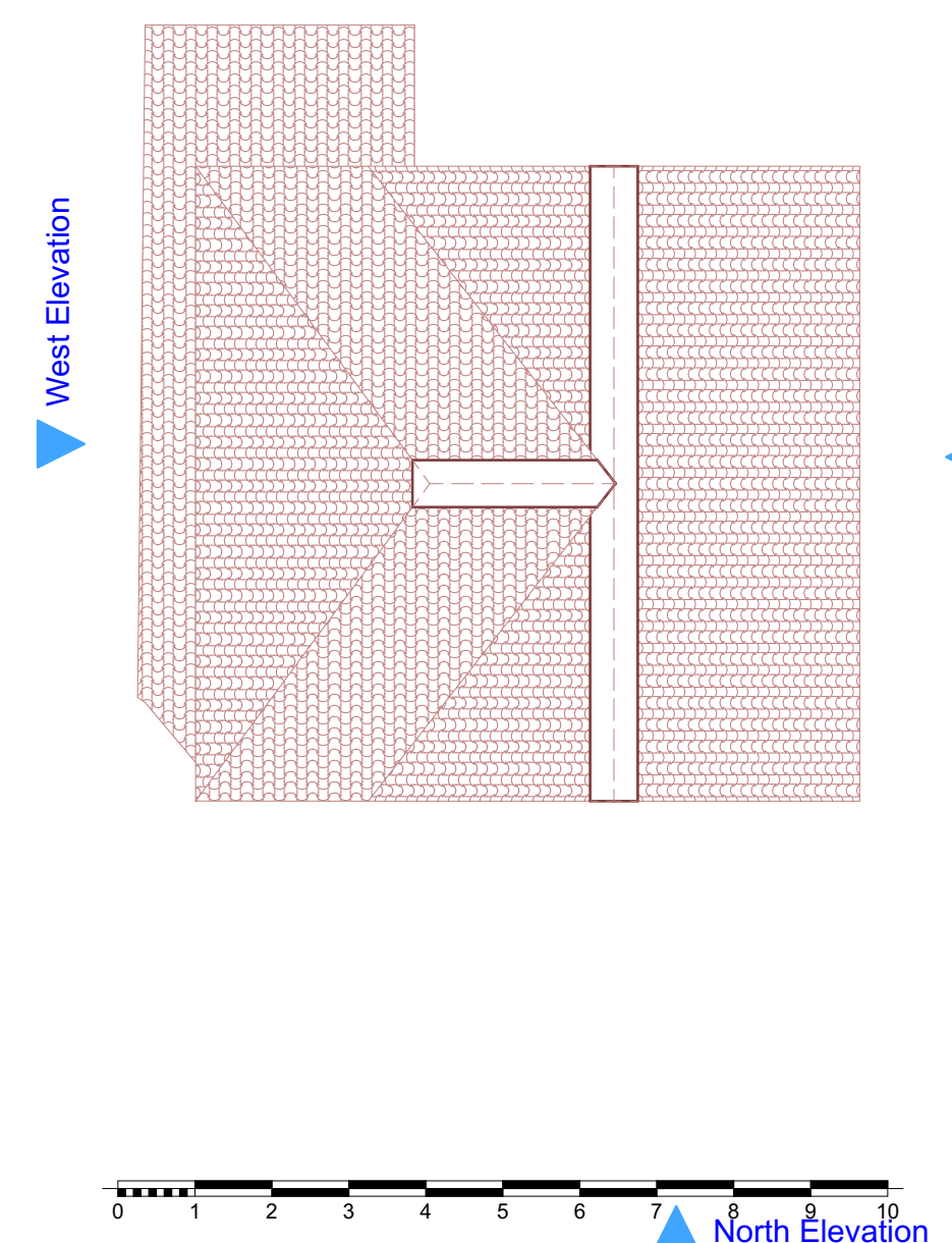
14 Roof Proposed 1:100
