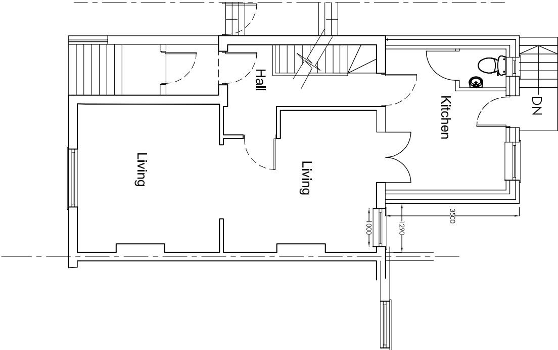
Proposed Ground Plan
