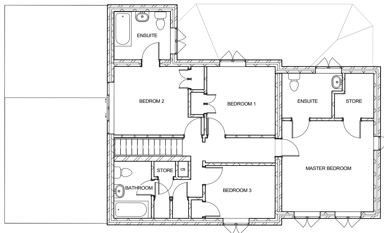
2 FIRST FLOOR 1 : 100
