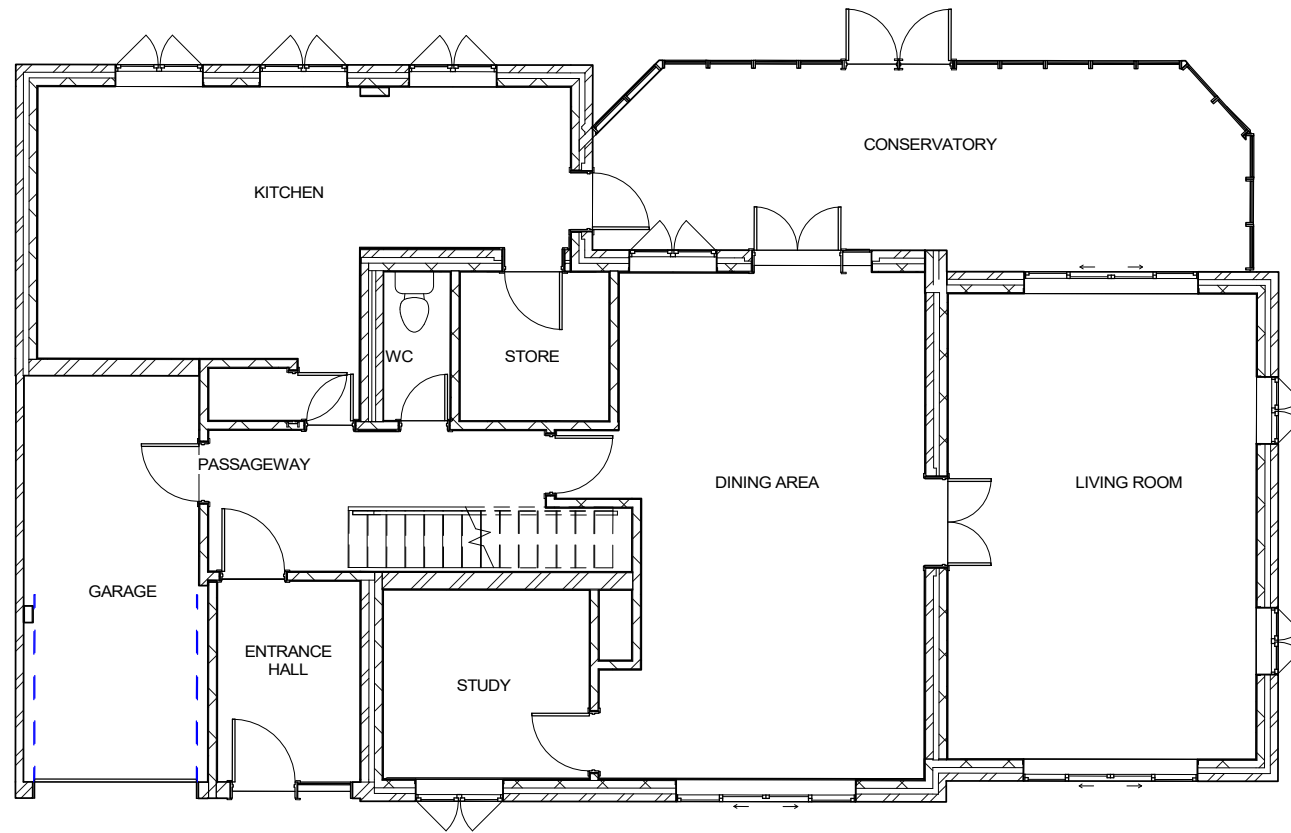
1 GROUND FLOOR 1 : 100
