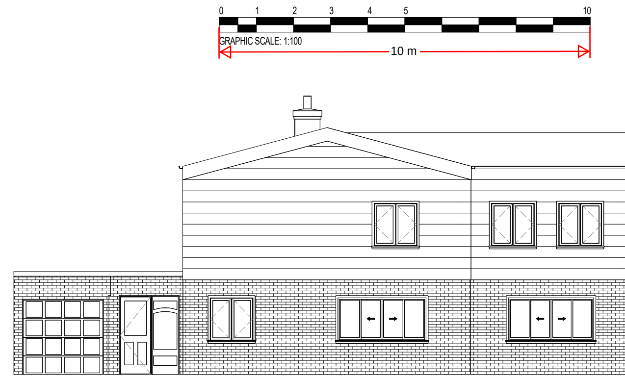
5 FRONT ELEVATION 1 : 100
