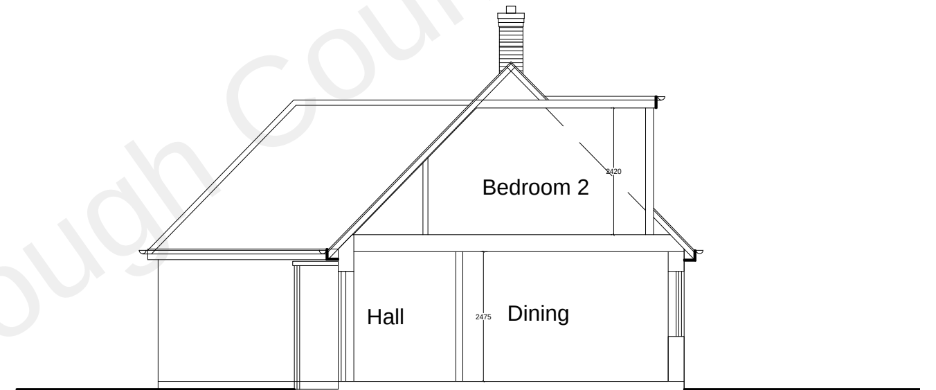
Typical Section
