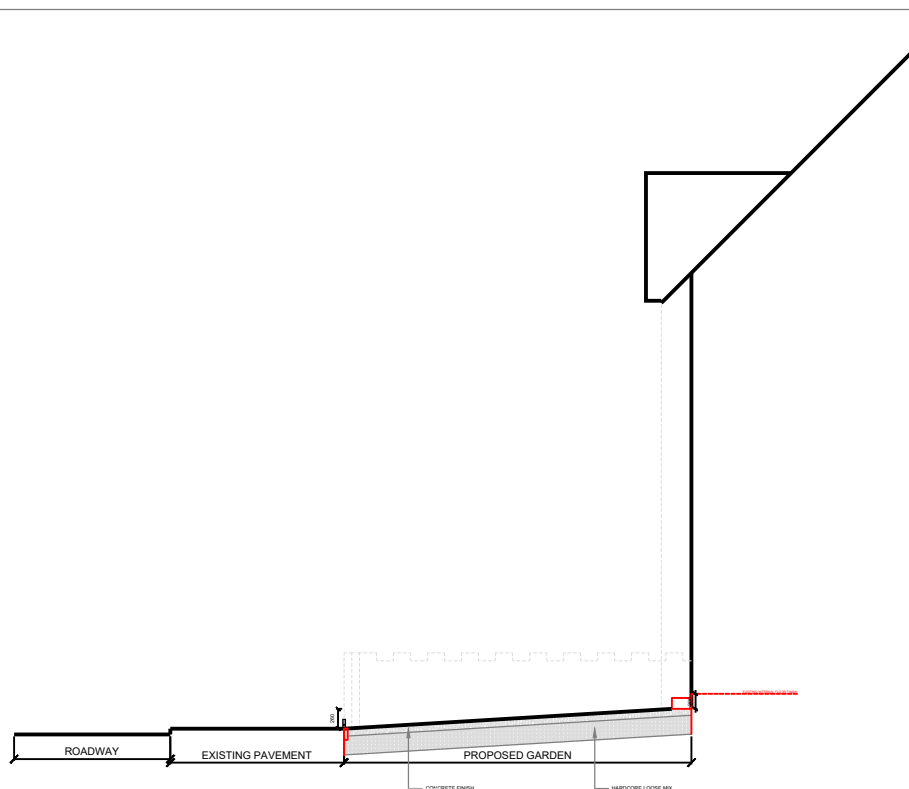
PROPOSED SECTION
