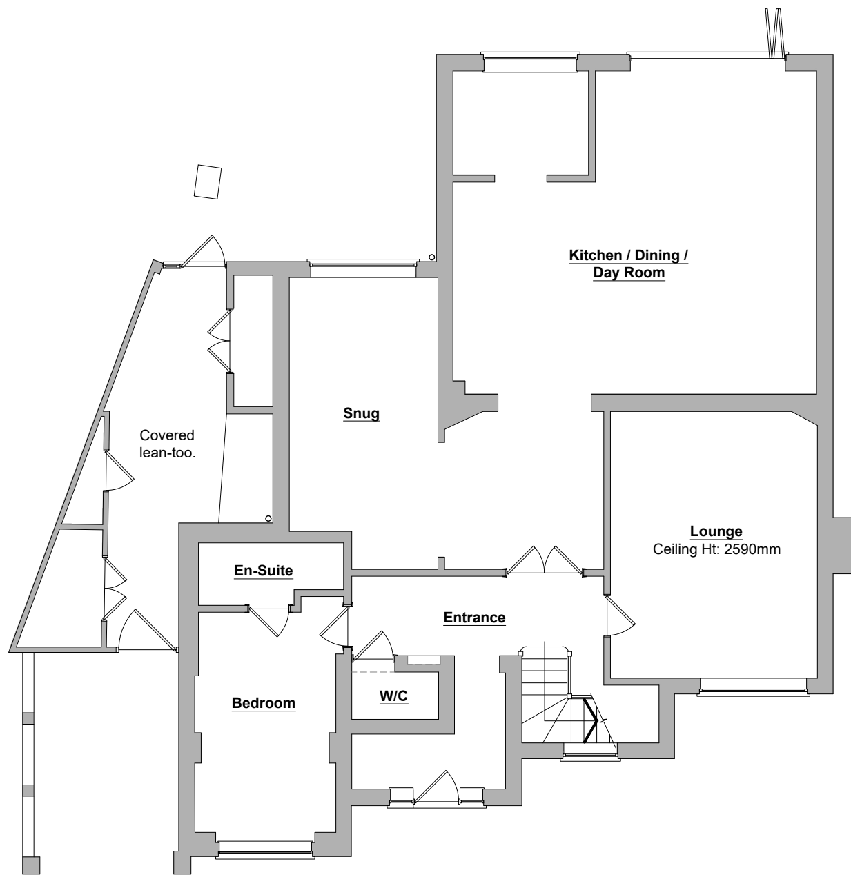
EXISTING GROUND FLOOR LAYOUT PLAN Scale 1/100
