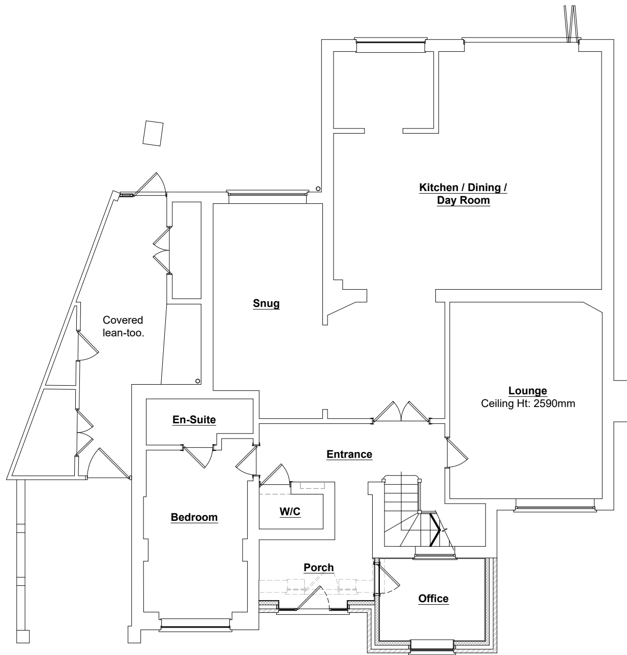
PROPOSED GROUND FLOOR LAYOUT PLAN Scale 1/100
