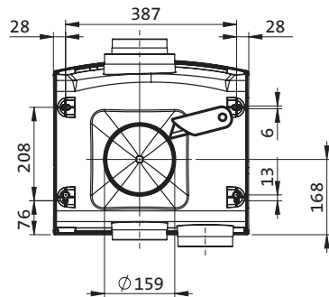
Fig. 4 Rear view with Ø 160 mm connection
