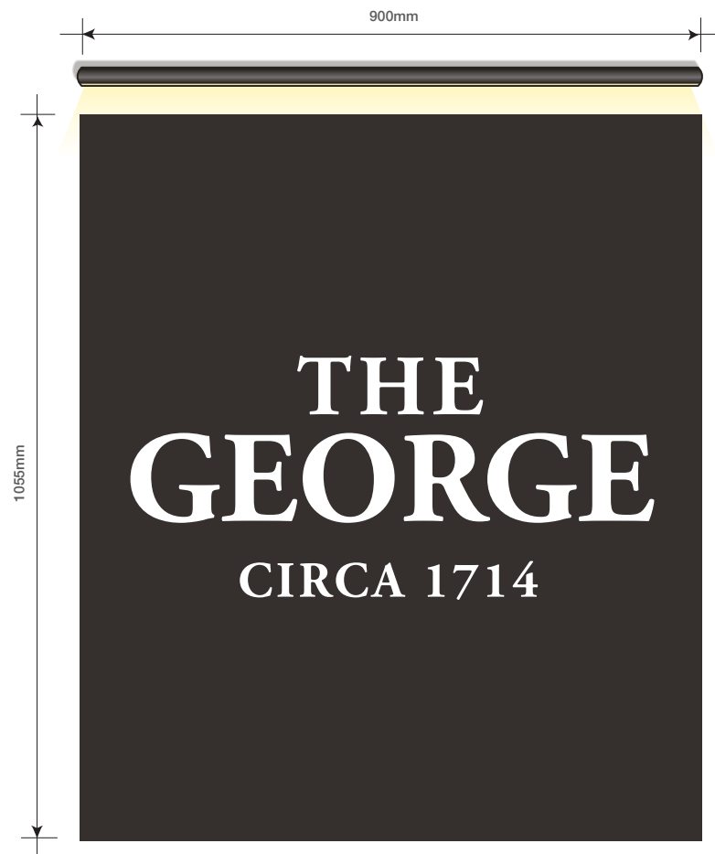
ITEM 3. Digital print on existing pictorial. Illuminated by new LED Trough lights. Scale 1:10 AGL: 3600mm MCH: 130mm
