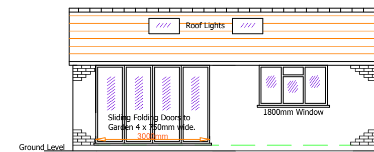
Proposed Side (East) Elevation 1:100
