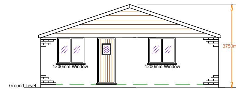
Proposed Front (North) Elevation 1:100
