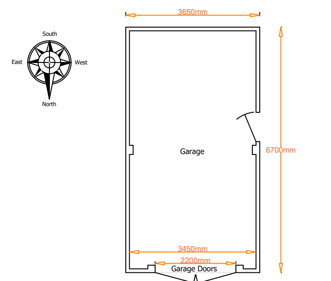
Existing Ground Floor Garage Plan 1:100
