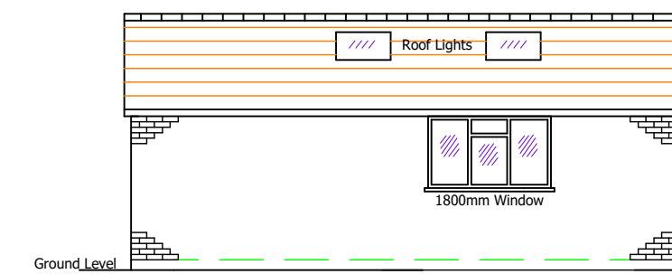
Proposed Side (West) Elevation 1:100
