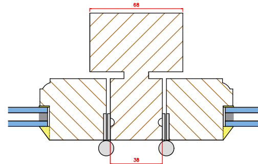
Sections – Mullion 1:2 @ A3
