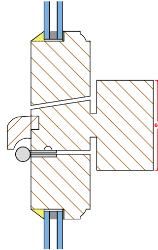
Sections – Jamb 1:2 @ A3
