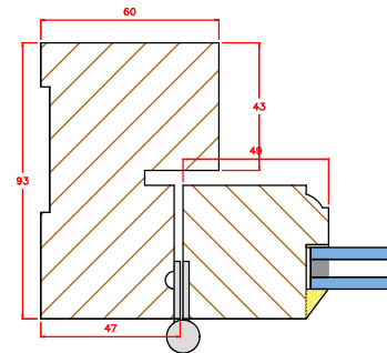
Sections – Jamb 1:2 @ A3
