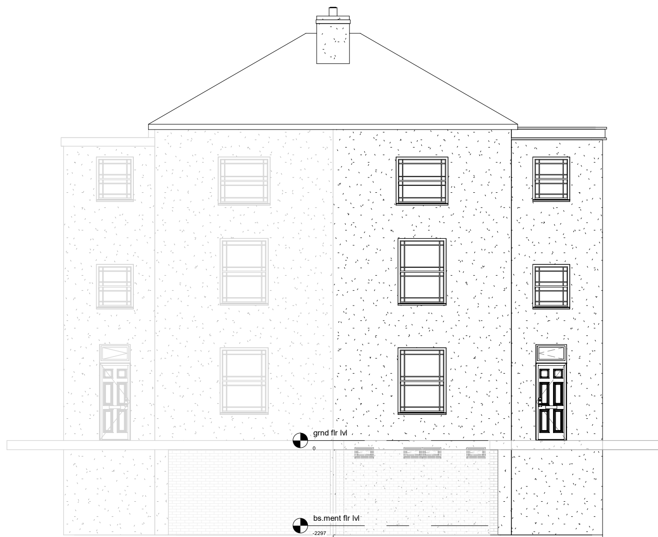
Existing Elevation-Front
