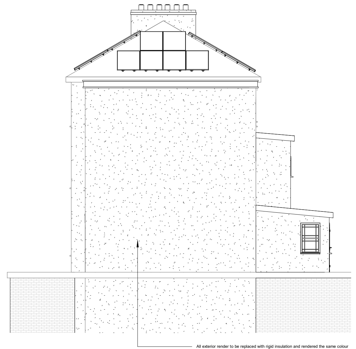
Proposed Elevation-Right side
