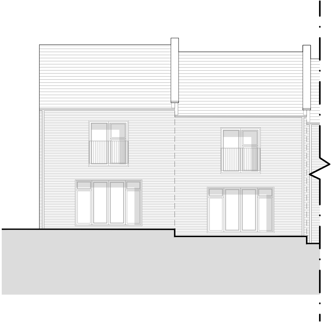
Rear Elevation @1:100
