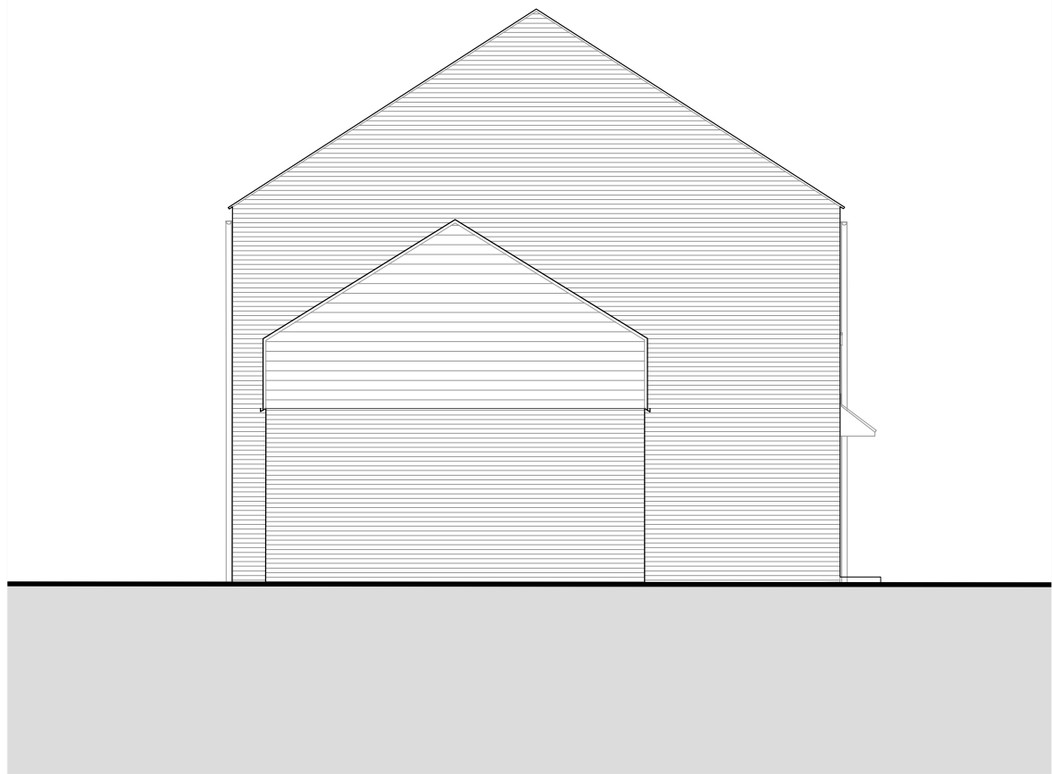
Side Elevation (1) @1:100
