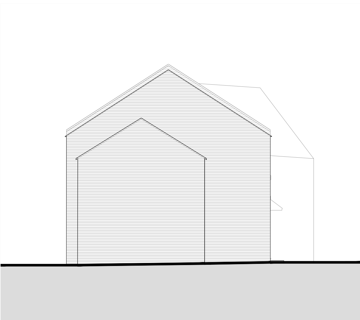
Side Elevation (1) @1:100
