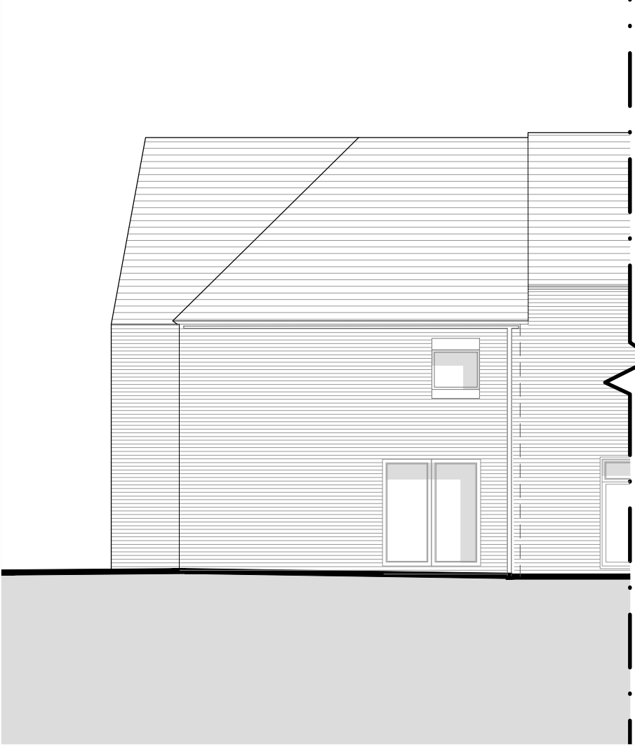
Rear Elevation @1:100
