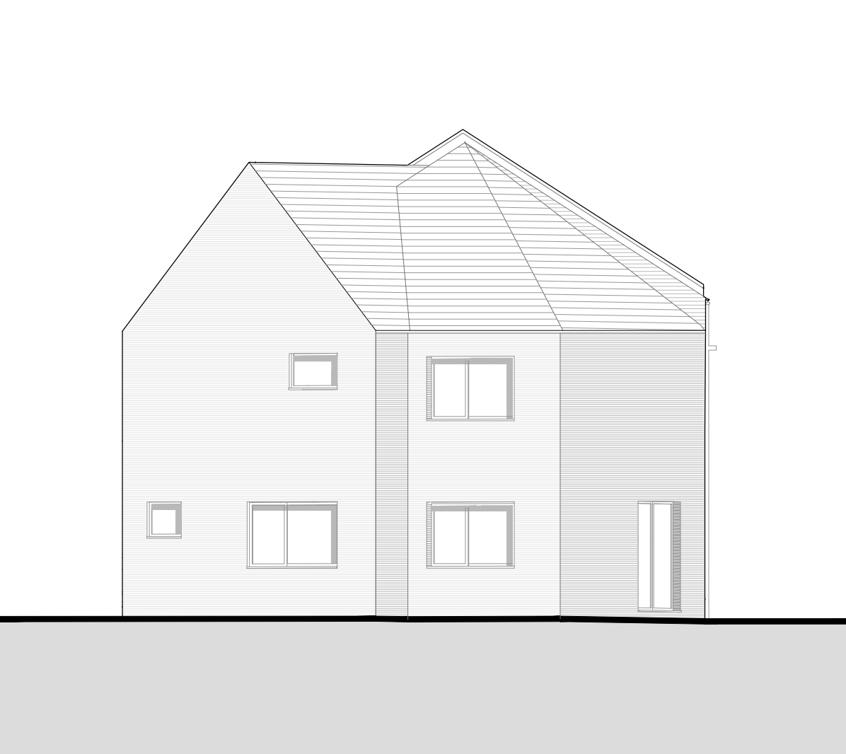
Side Elevation (2) @1:100
