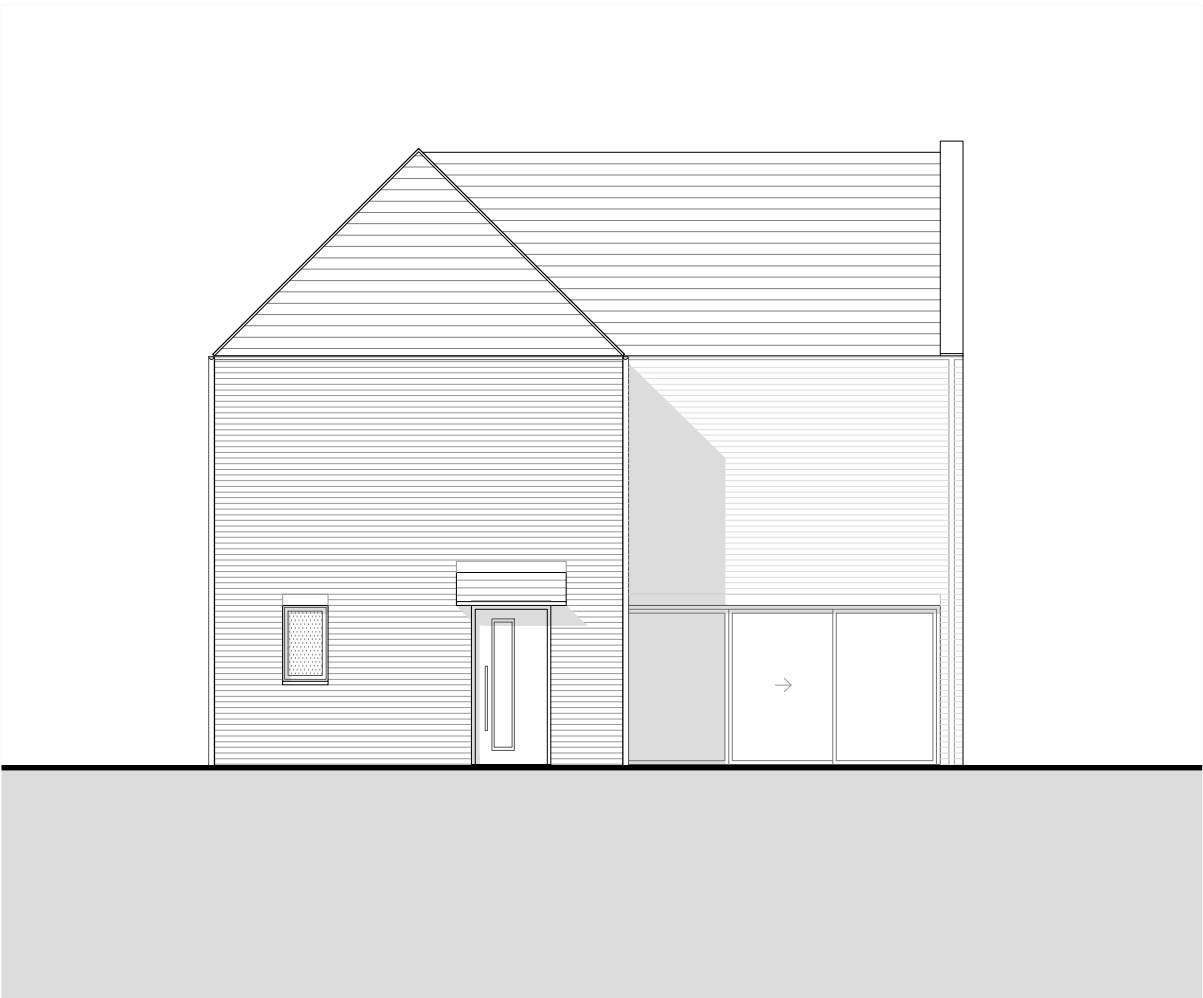
Front Elevation @1:100
