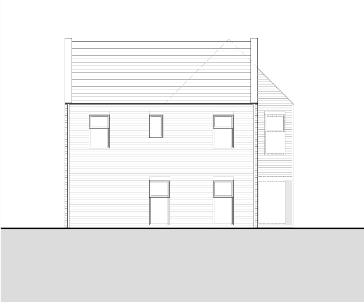
Rear Elevation @1:100
