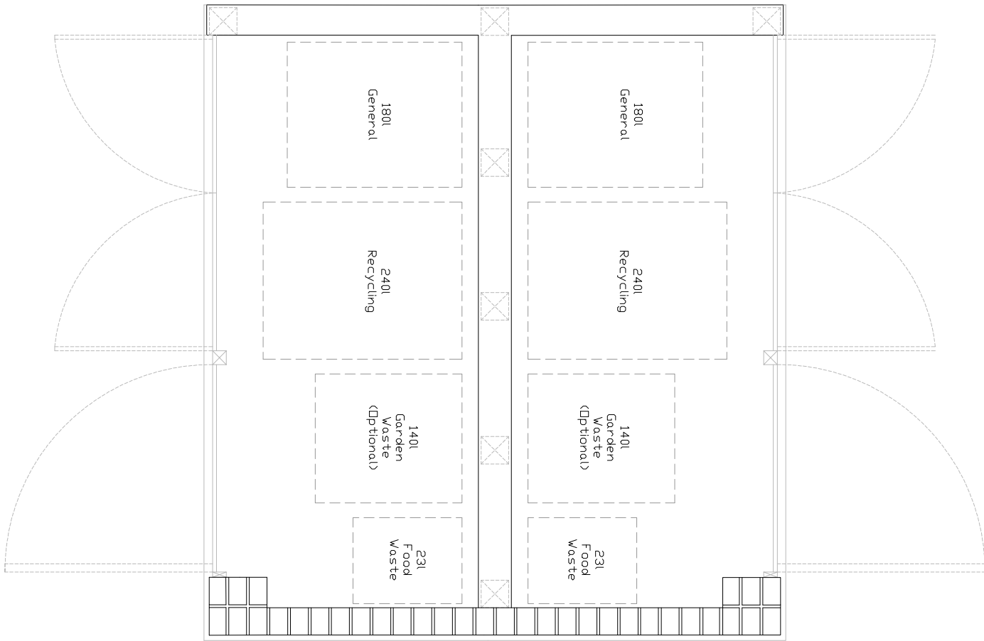
Plan @1:20
