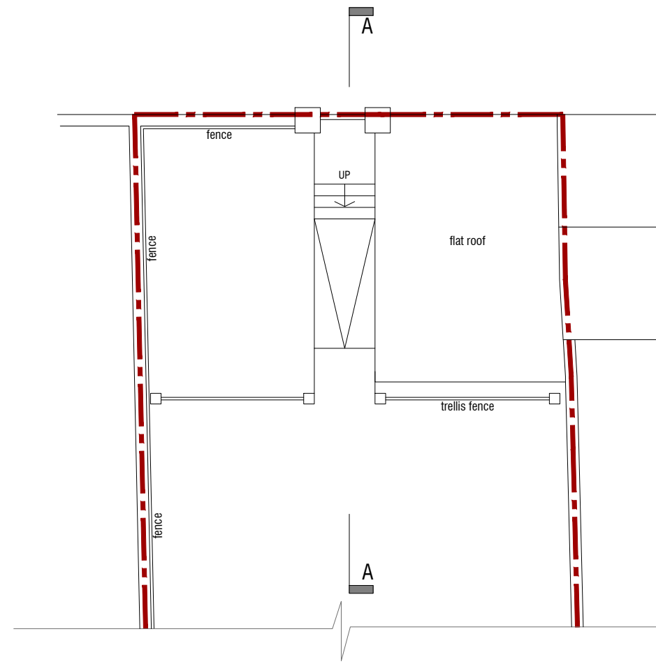
EXISTING ROOF PLAN Scale 1:100
