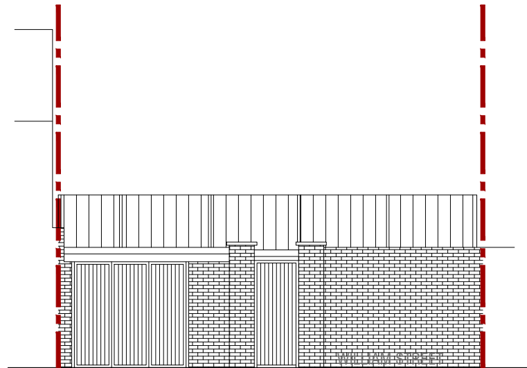
EXISTING ELEVATION (E1) Scale 1:100
