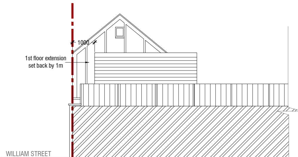
PROPOSED ELEVATION (E4)
