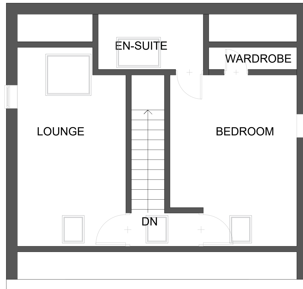
Existing Loft Plan
