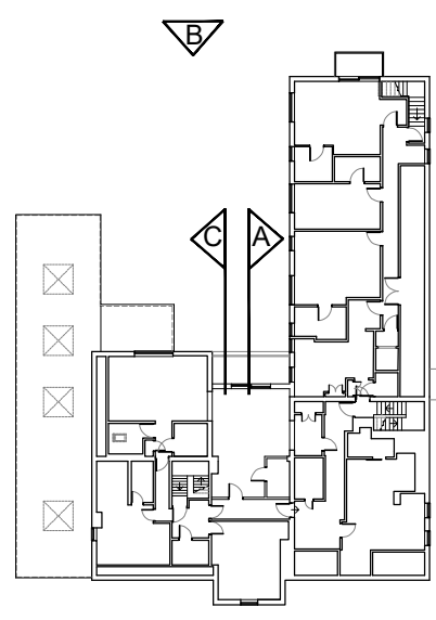
PROPOSED SECOND FLOOR KEY PLAN 1:500
