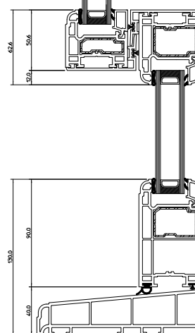
Sideways View - Deep Bottom Rail
