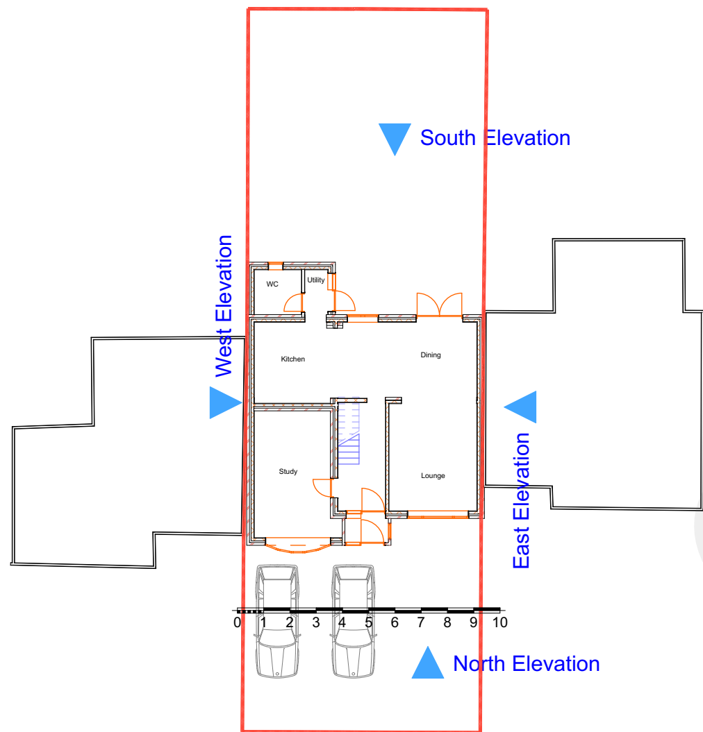
3 Site Plan Proposed 1:200
