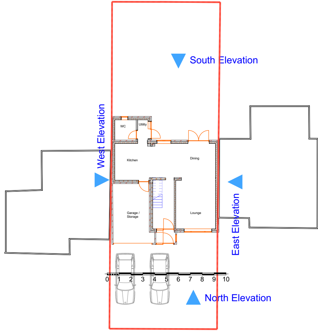
2 Site Plan Existing 1:200
