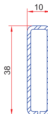
Article No 113.041 1.0mm Steel
