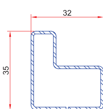
Article No 113.371 1.2mm Steel Door Frame Locking Side
