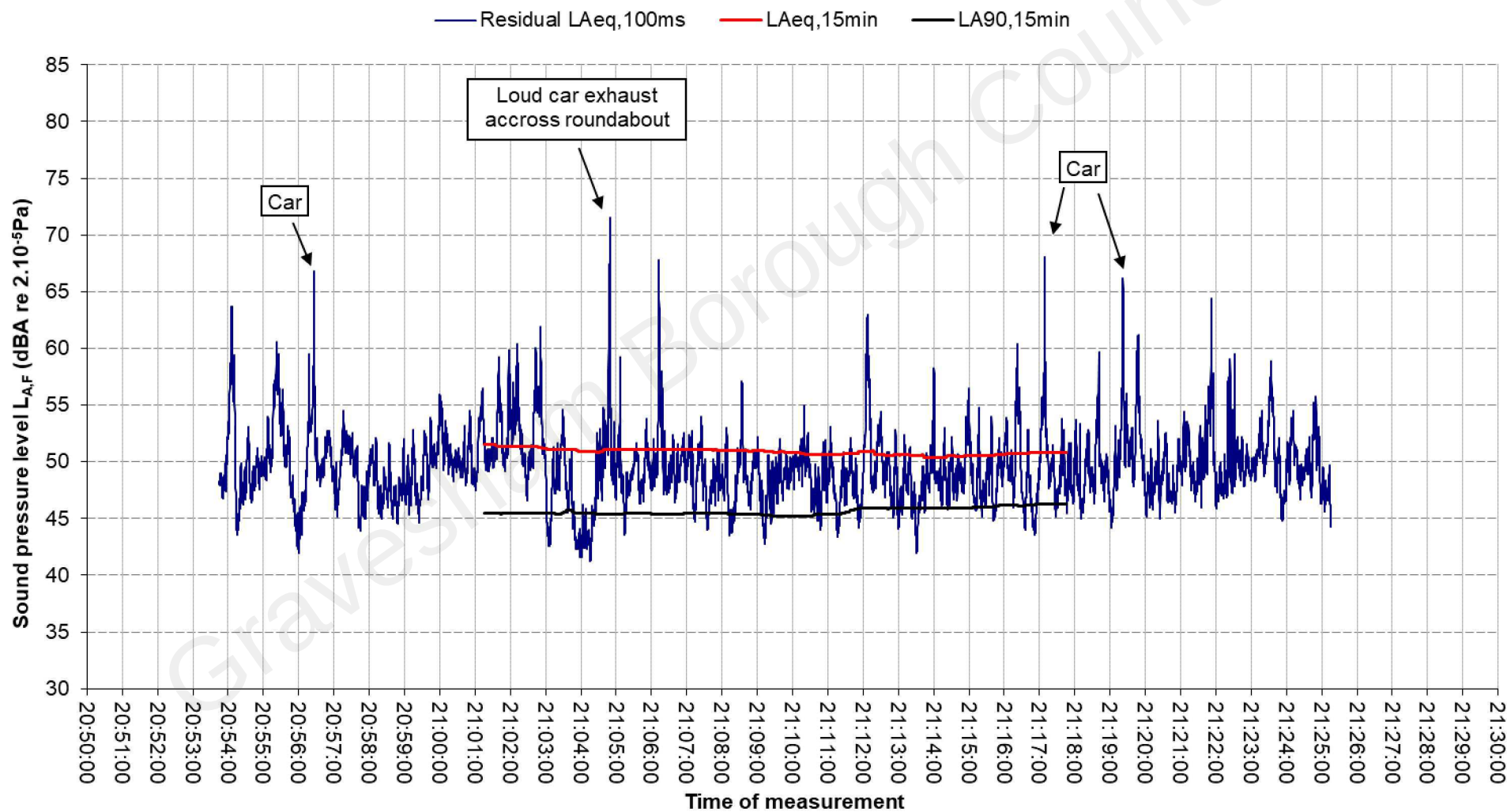
Graph 1 - Existing ambient sound level in vicinity of Morrisons Gravesend Measured 15 th July 2021
