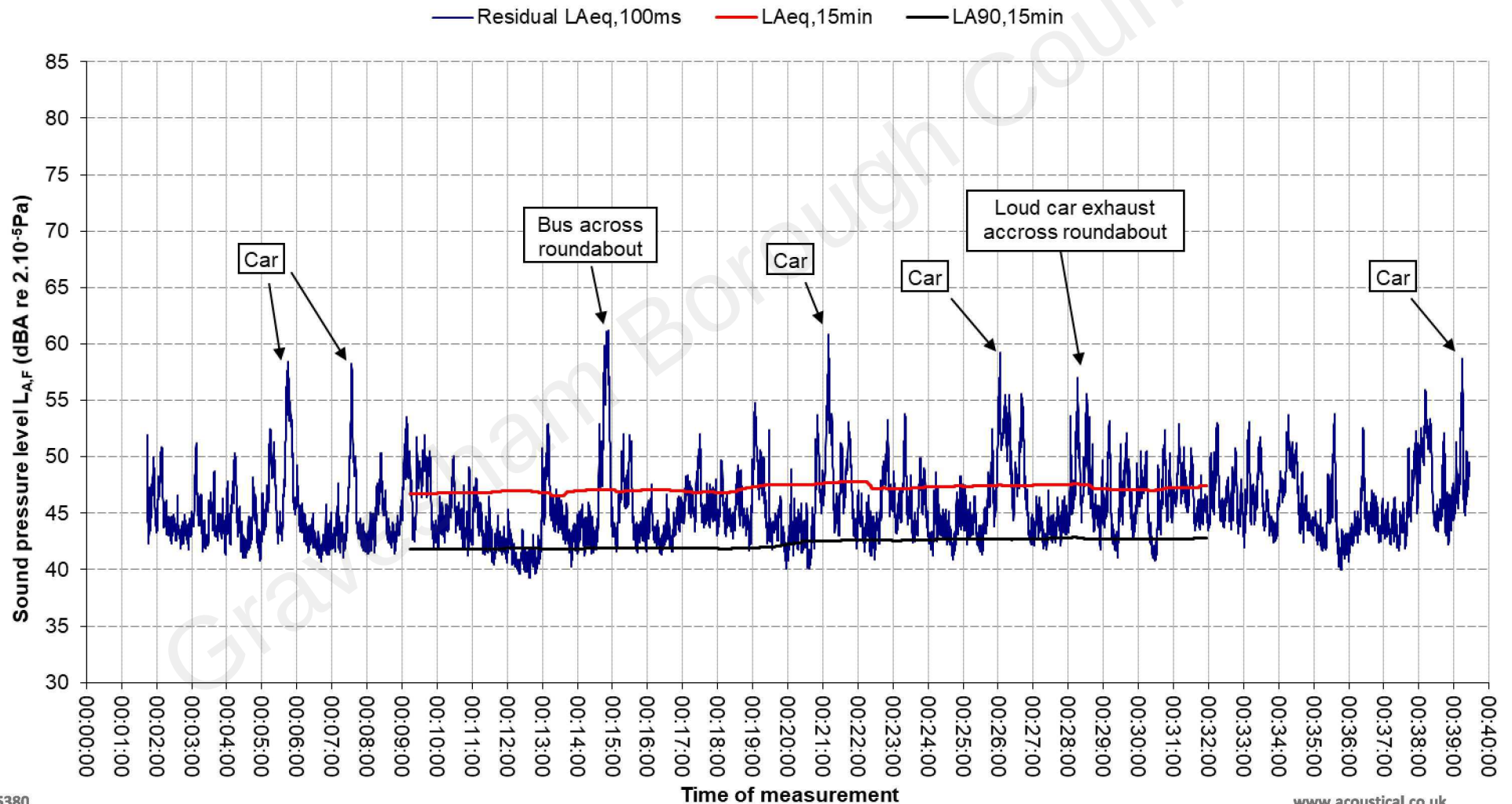
Graph 2 - Existing ambient sound level in vicinity of Morrisons Gravesend Measured 15 th July 2021
