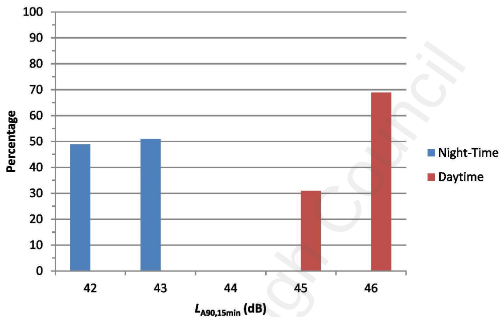
Figure 7.3 Histogram of background sound levels ( L_{A90,15min} )
