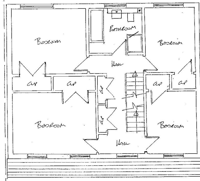
EXISTING First Floor GA
