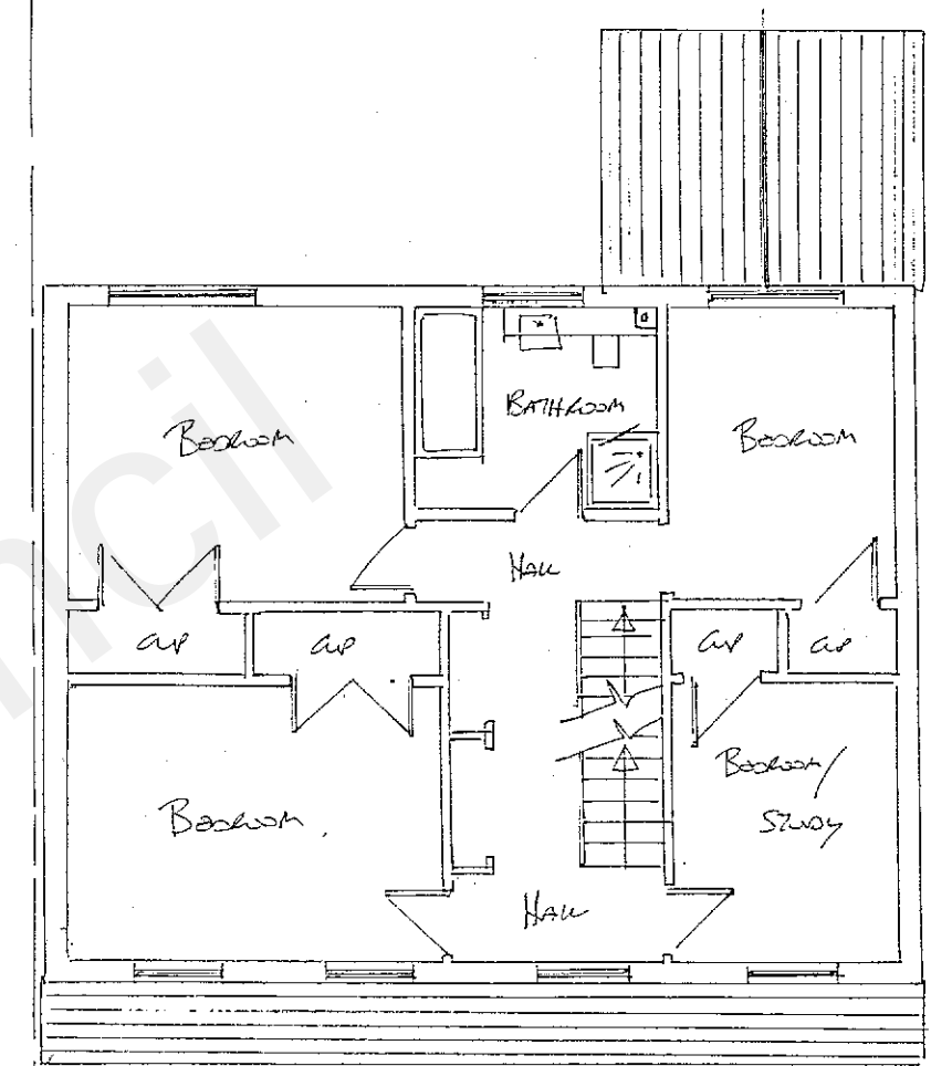
PROPOSED First Floor GA
