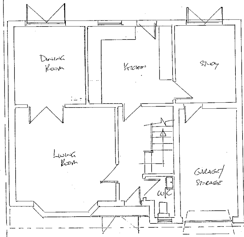
EXISTING Ground Floor GA
