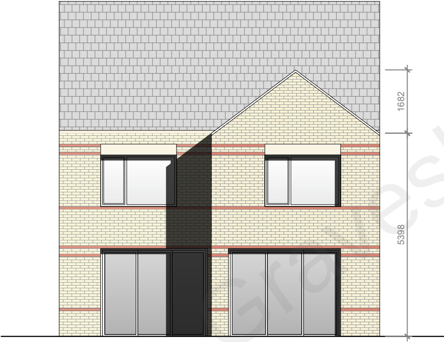
Indicative Rear Elevation
