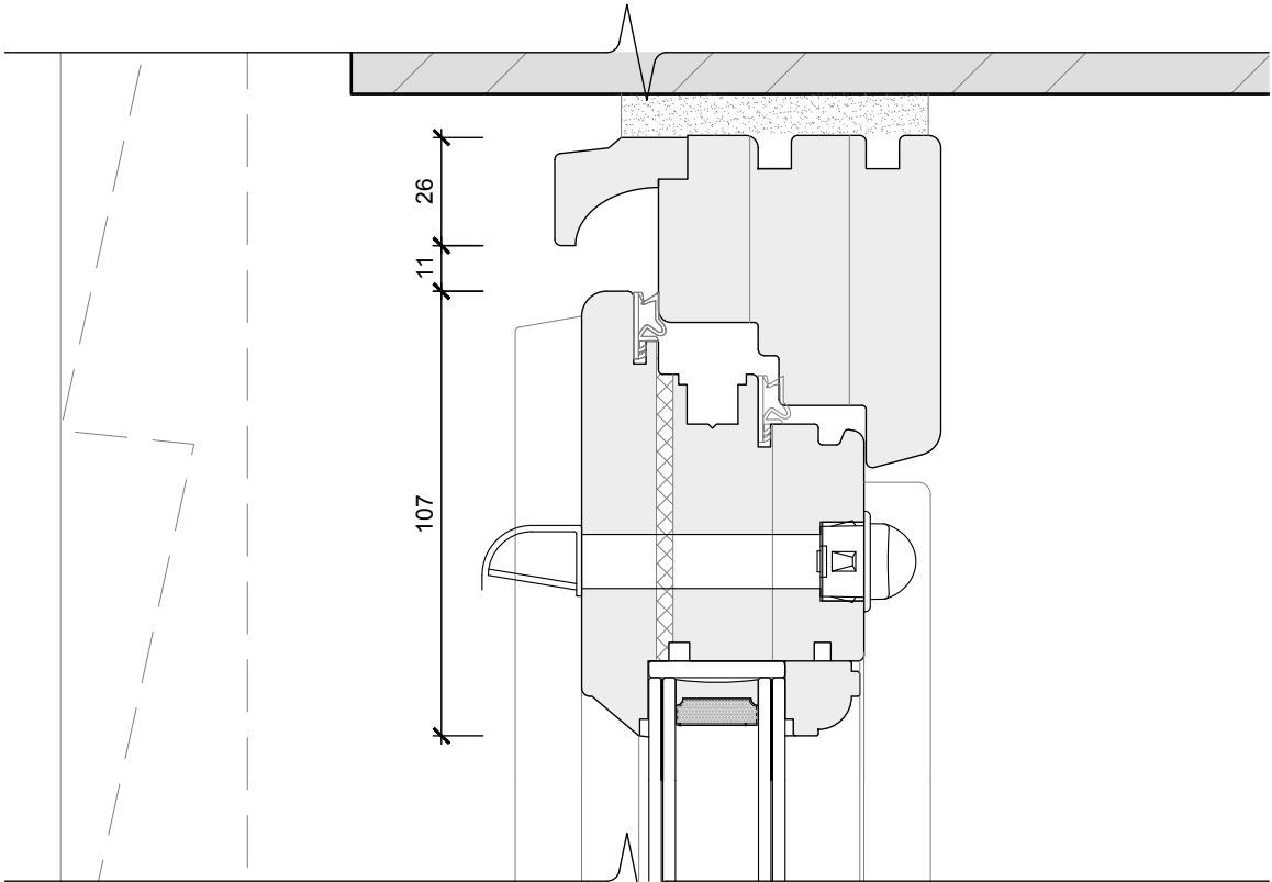
Proposed Head Detail 1:2
