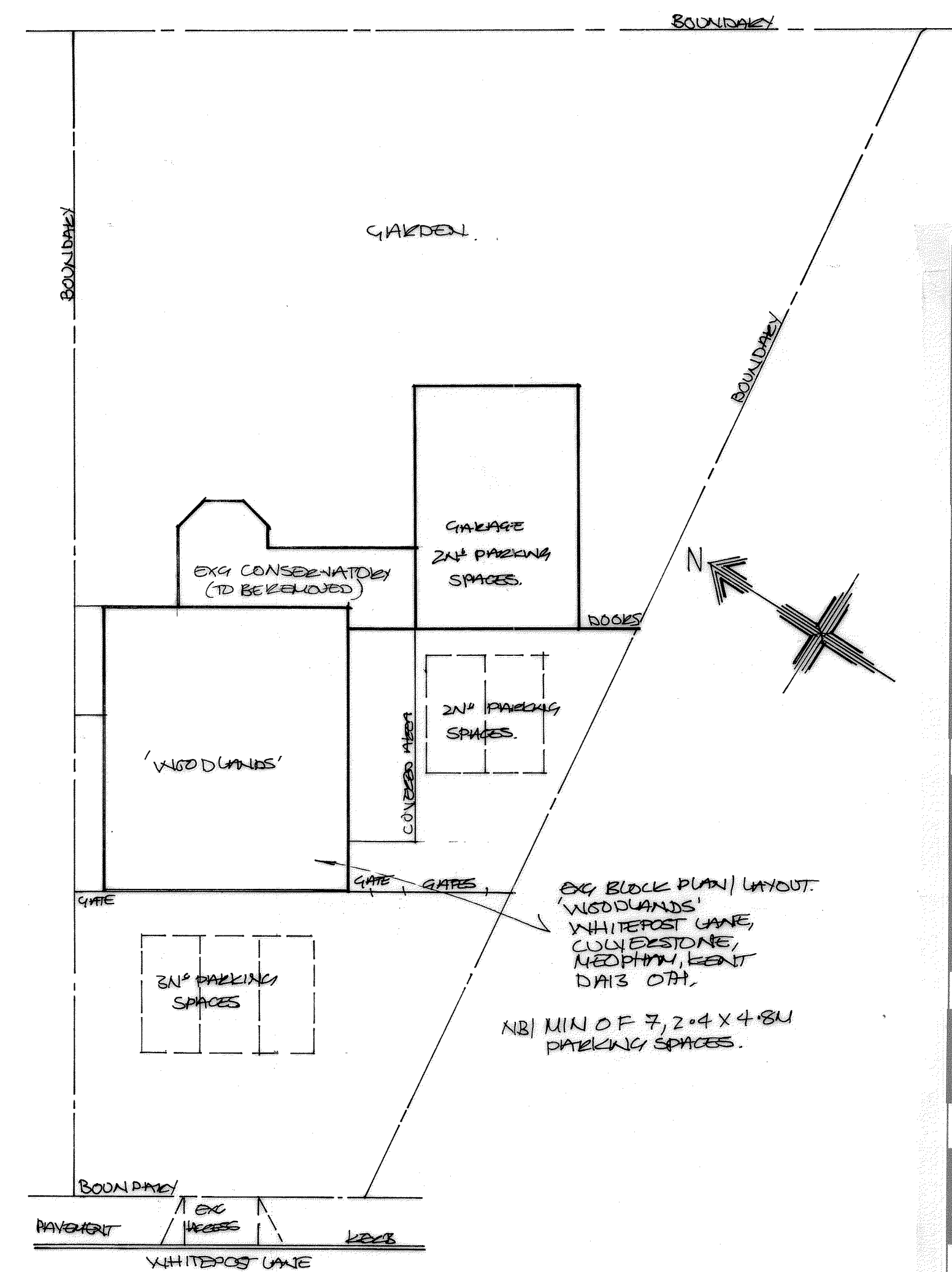
Exg. Block Plan.
