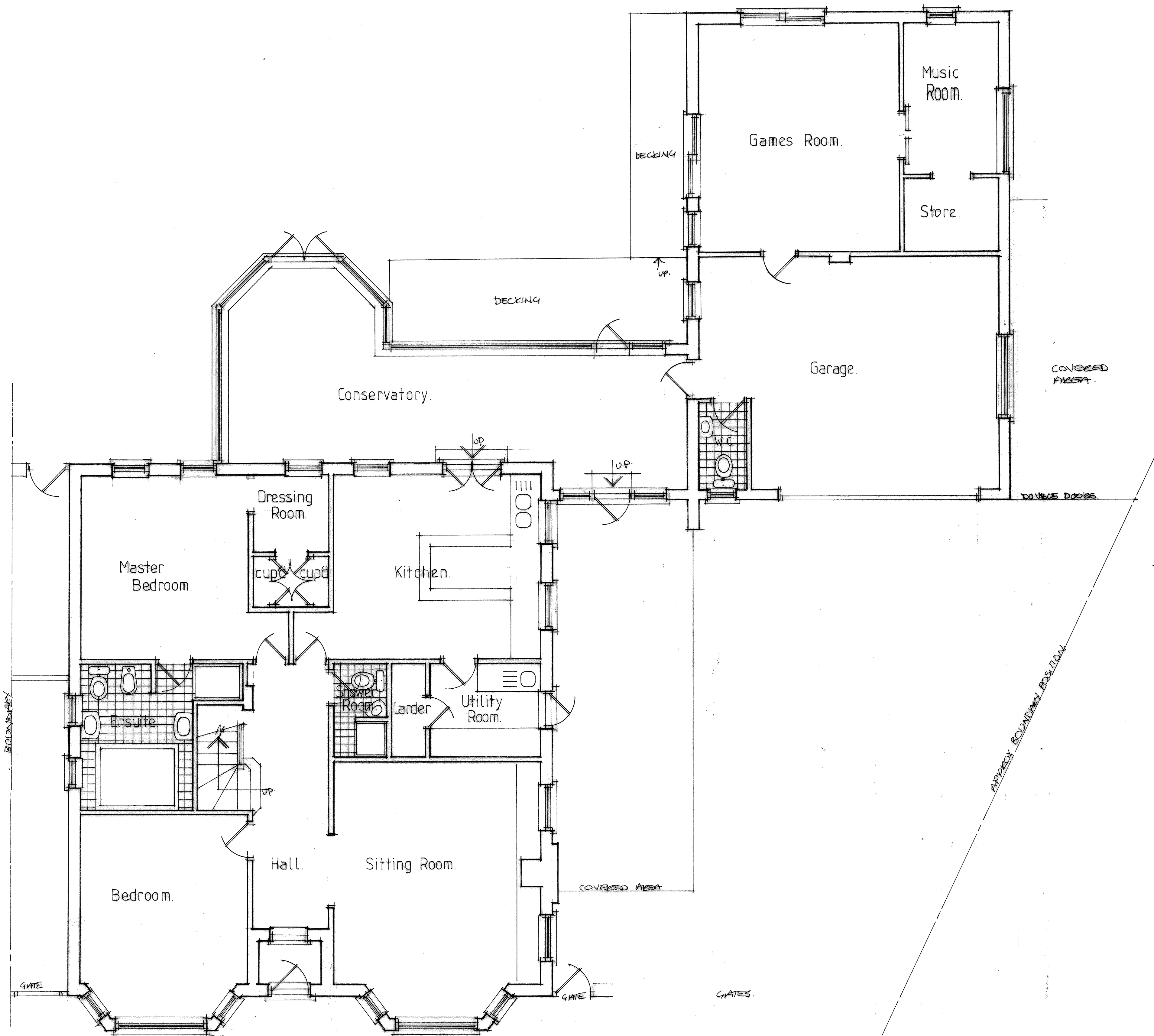
Existing Ground Floor Layout.
