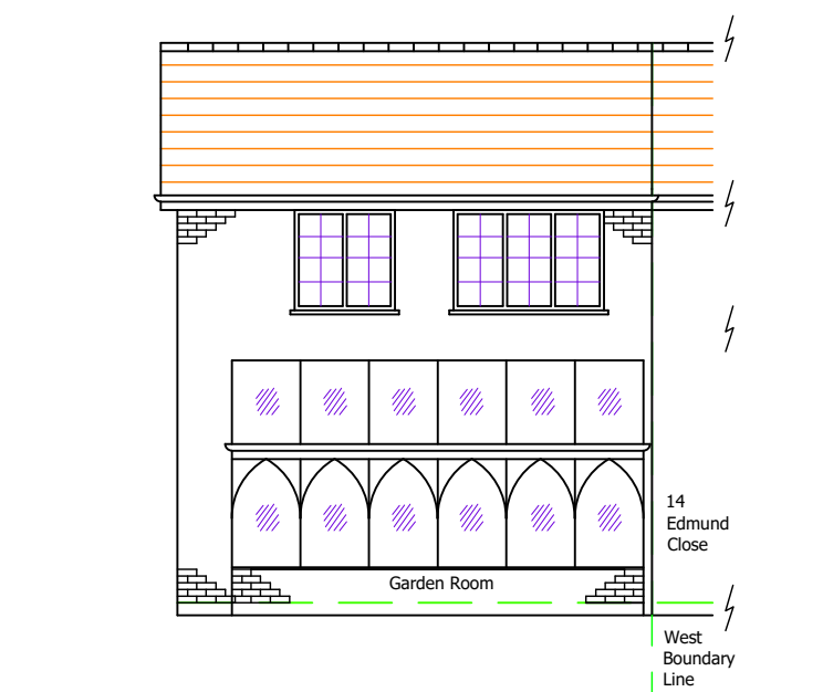
Existing Rear (North) Elevation 1:100
