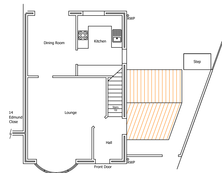
Proposed Extension Roof Tile Plan
