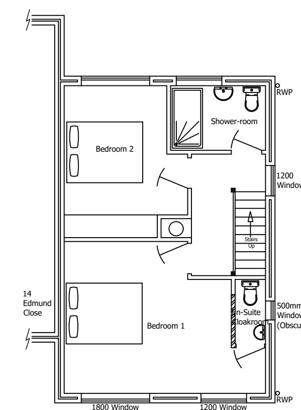
Proposed First Floor Plan 1:100 Cloak-room to Bedroom 1
