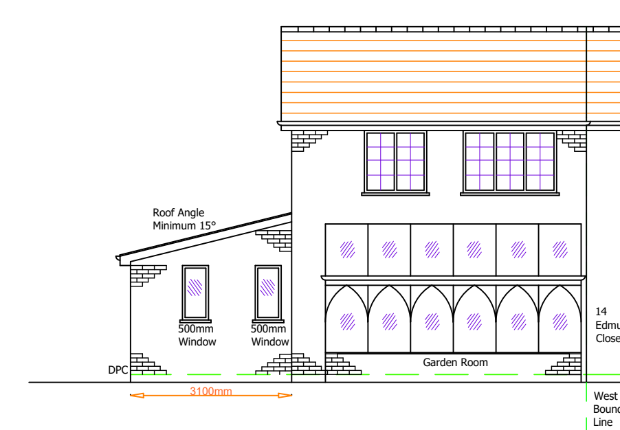
Proposed Rear (North) Elevation 1:100
