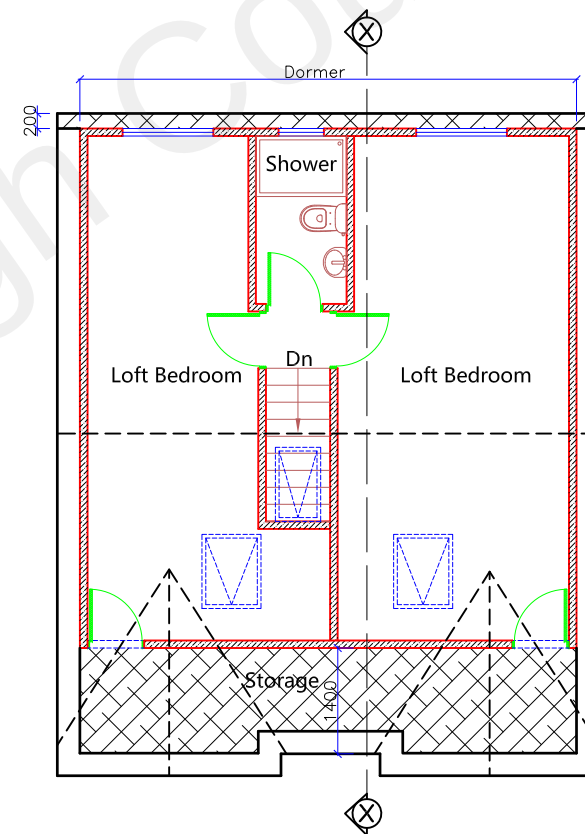
Proposed Loft Plan
