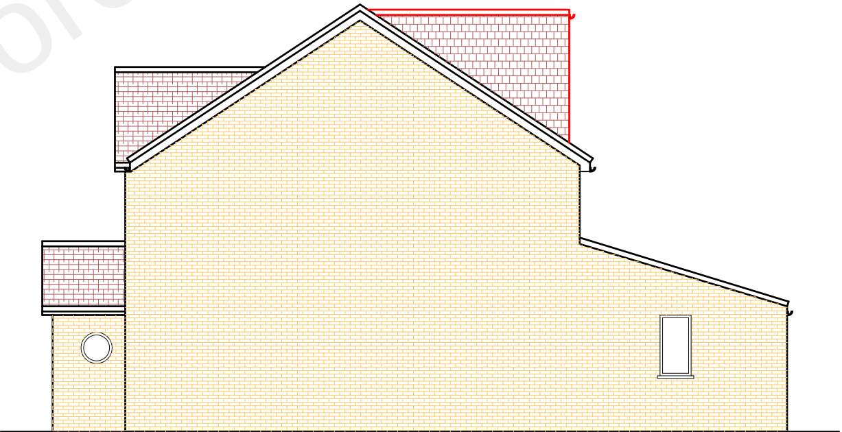
Proposed Side Elevation - B
