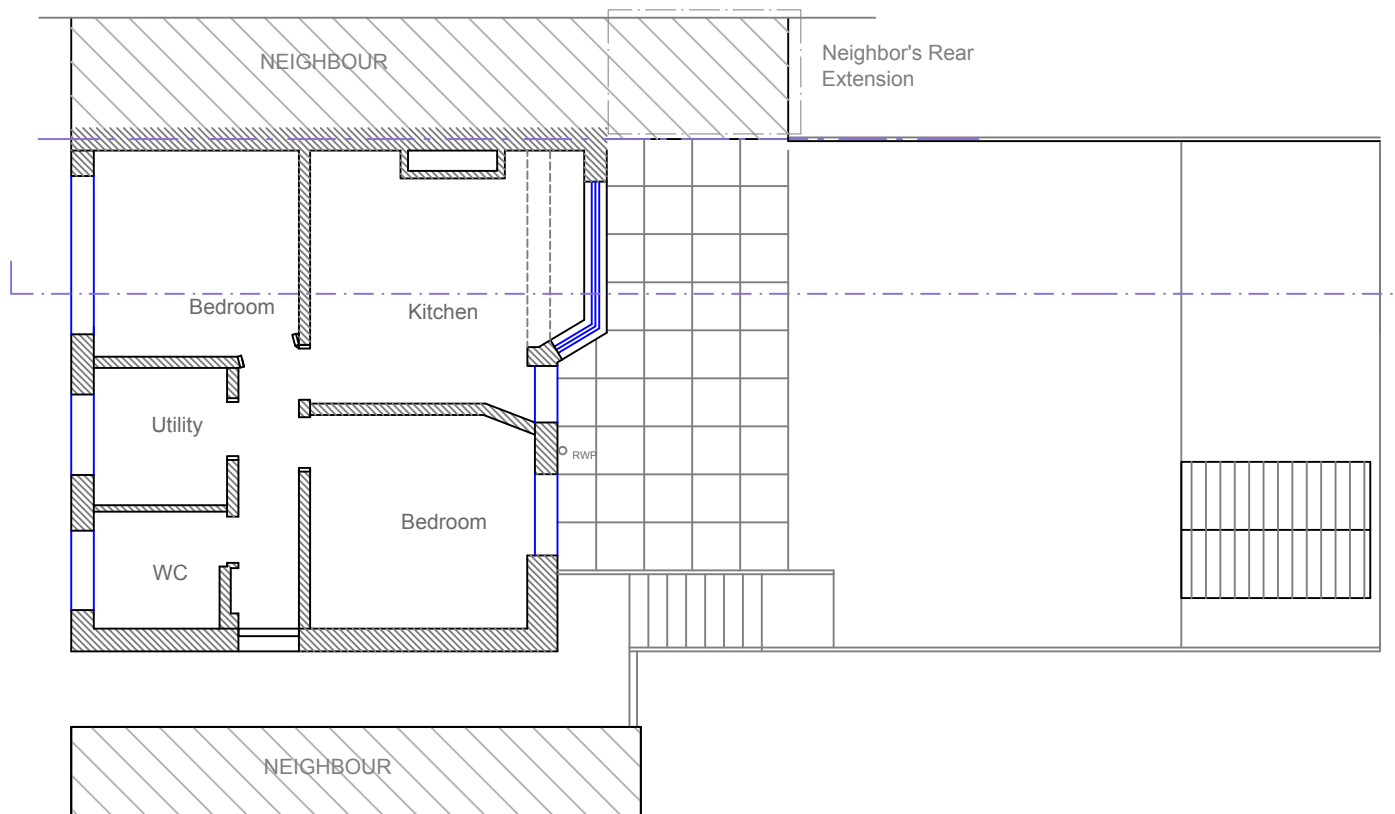
FLOOR PLAN
