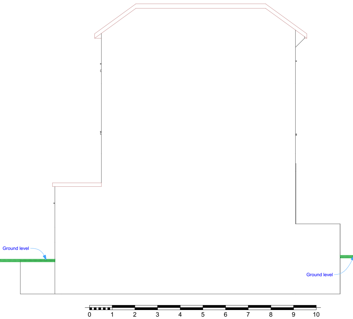
North Elevation Existing 1:100
