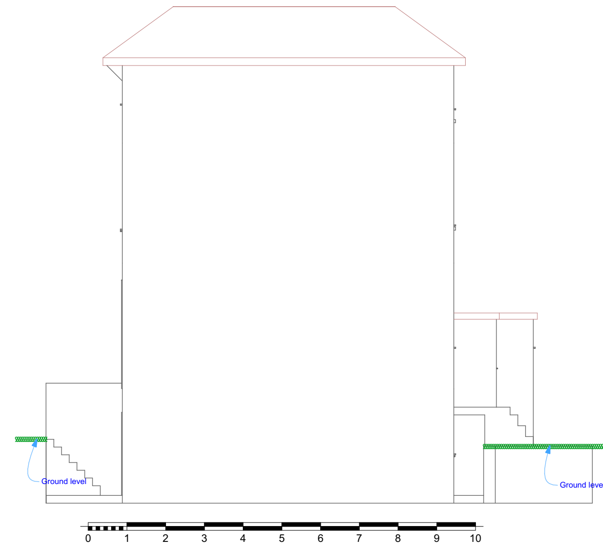
South Elevation Existing 1:100
