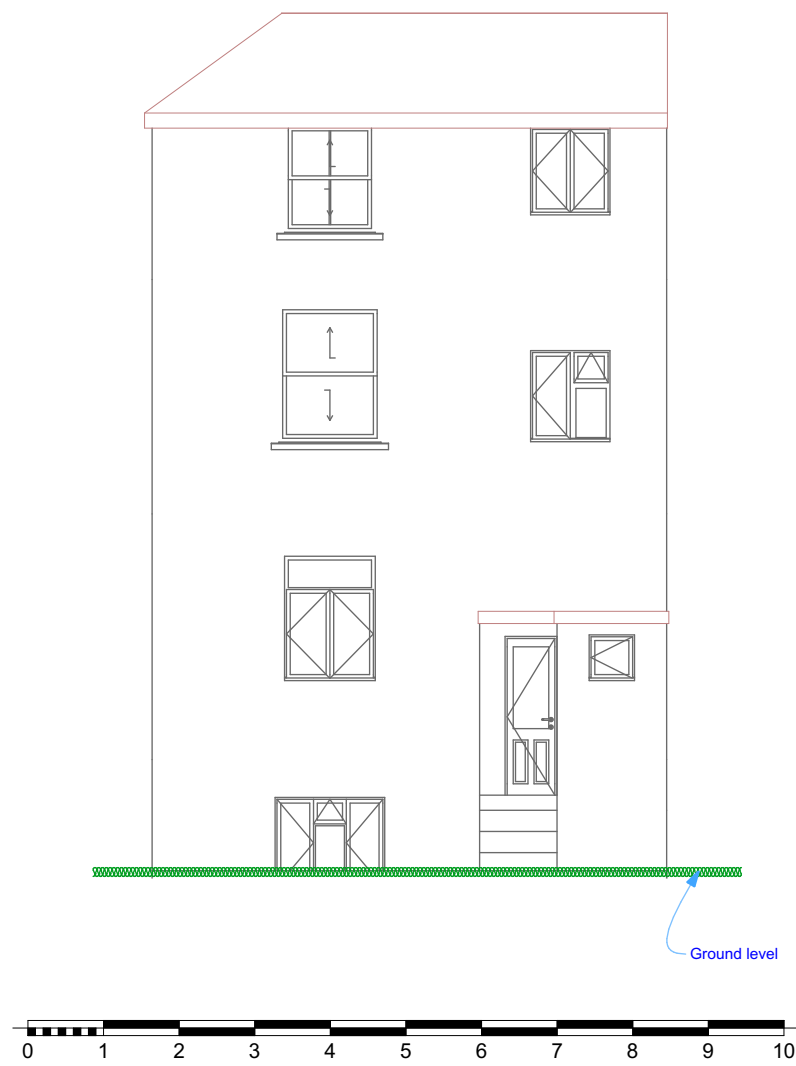
East Elevation Existing 1:100
