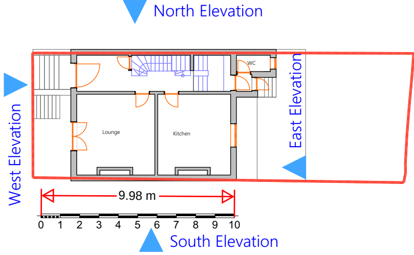
2 Site Plan Existing 1:200
