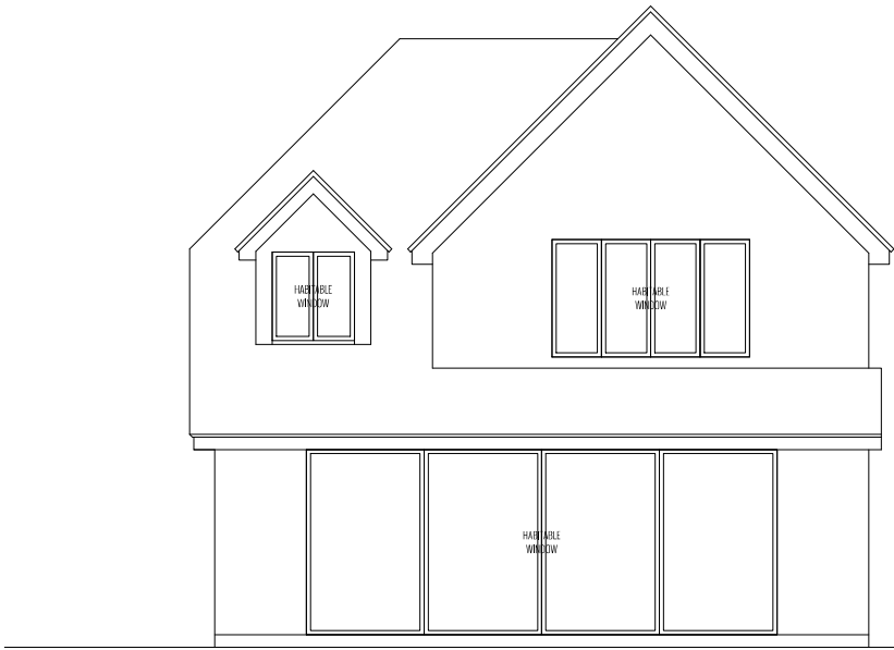
EAST ELEVATION
