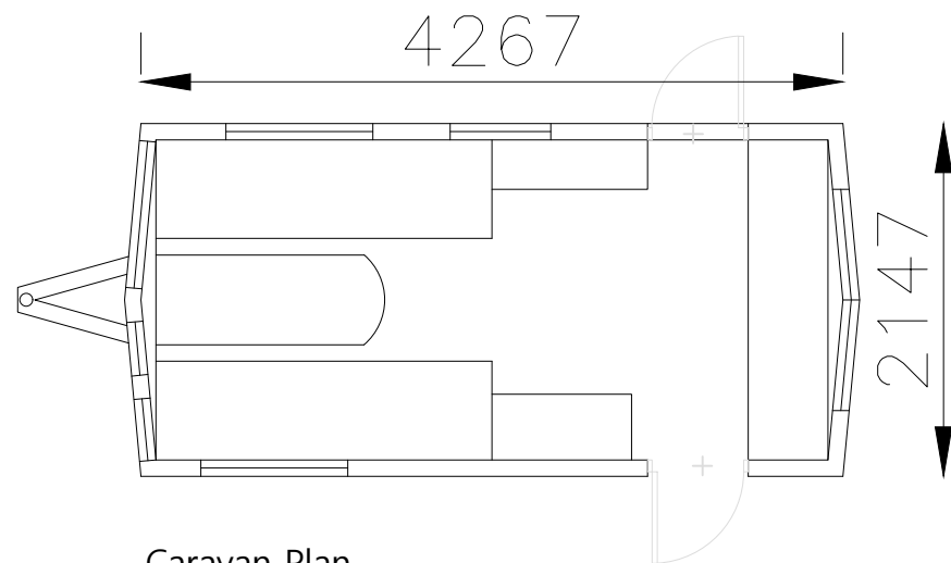
Caravan Plan
