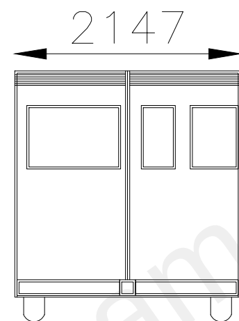
East Elevation
