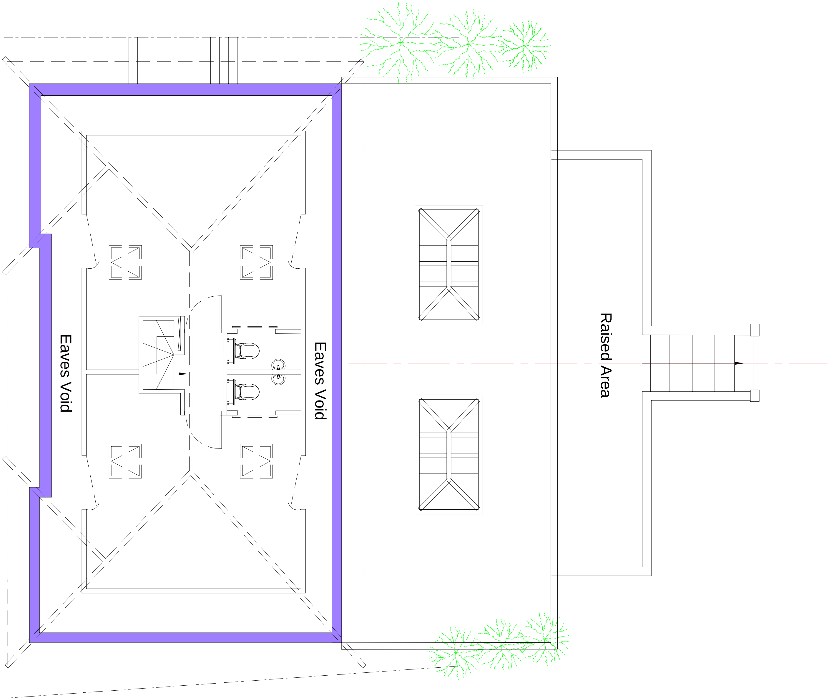
Proposed Loft Plan
