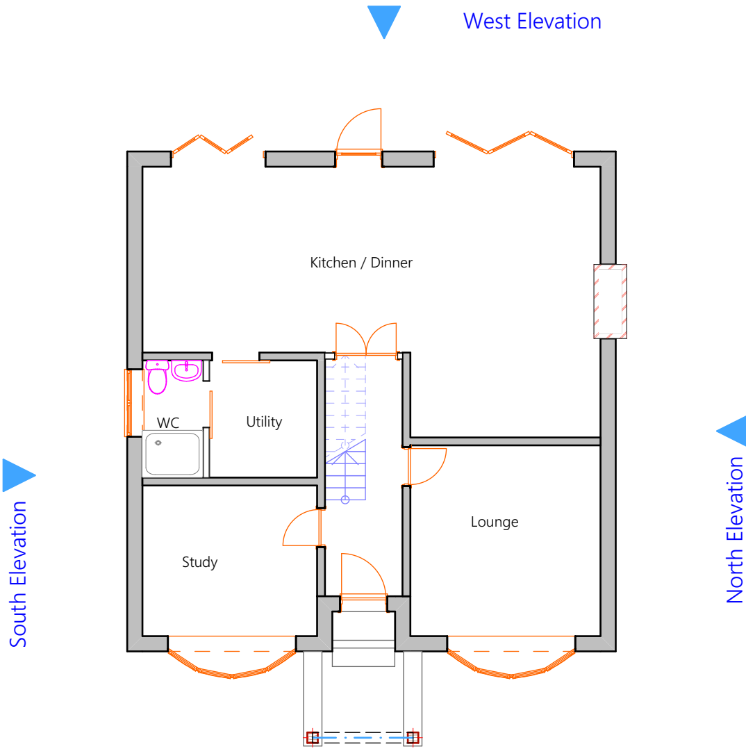
10 GF Ground Floor Proposed 1:100
