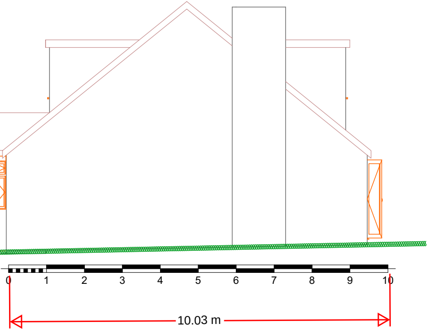
8 North Elevation Proposed 1:100
