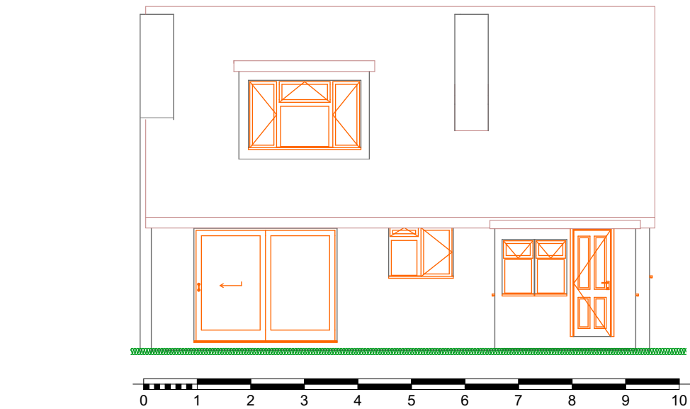
2 West Elevation Existing 1:100
