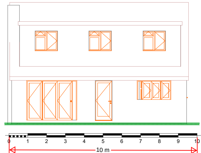
7 West Elevation Proposed 1:100
